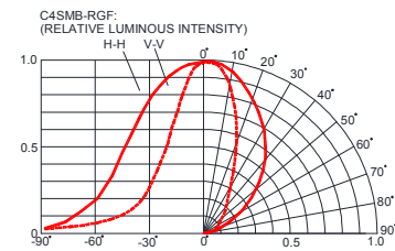
FIG.6b RED FAR FIELD PATTERN
