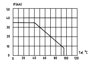
FIG.4b BLUE & GREEN MAXIMUM FORWARD DC CURRENT VS. AMBIENT TEMPERATURE ( T_{jmax}=105\text{ }^{\circ}\text{C} )
