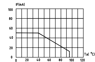
FIG.4a RED MAXIMUM FORWARD DC CURRENT VS. AMBIENT TEMPERATURE ( T_{jmax}=105\text{ }^{\circ}\text{C} )
