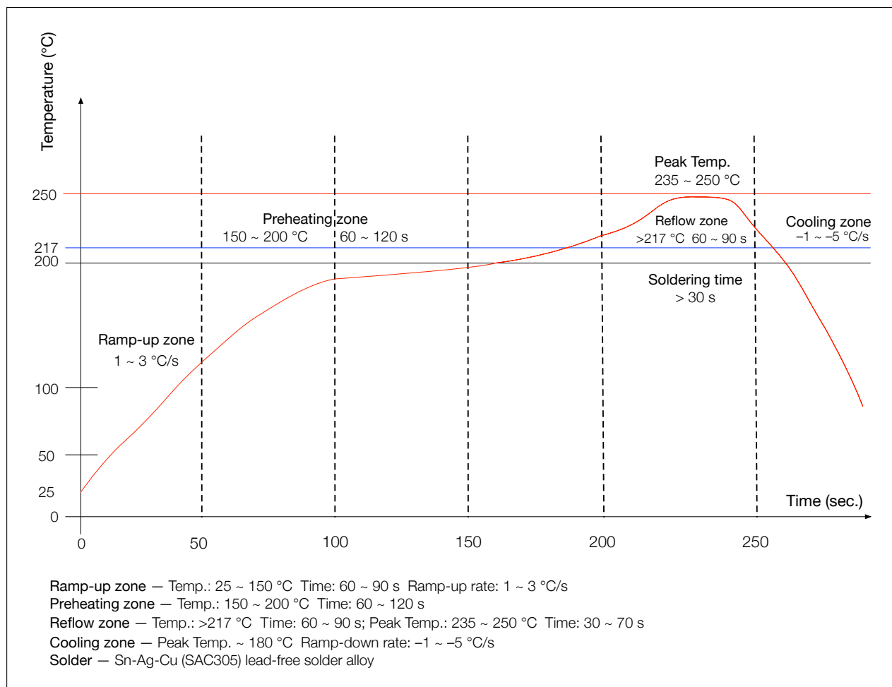
Figure 15: Reflow Profile
