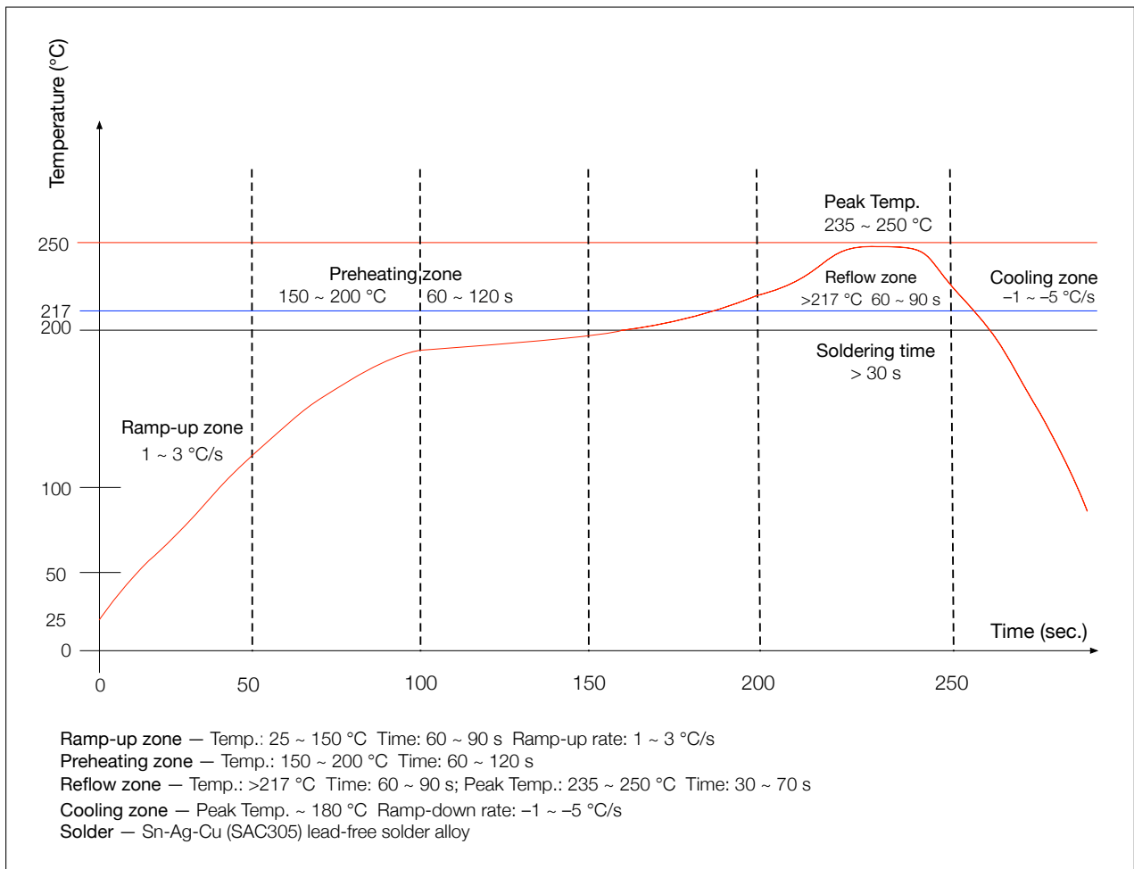
Figure 10: Reflow Profile
