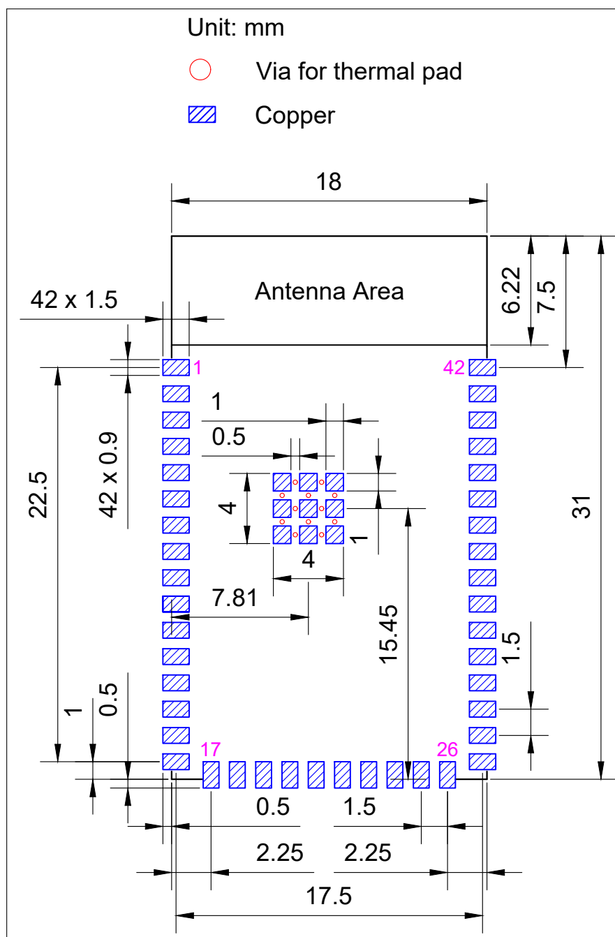
Figure 10: Recommended PCB Land Pattern
