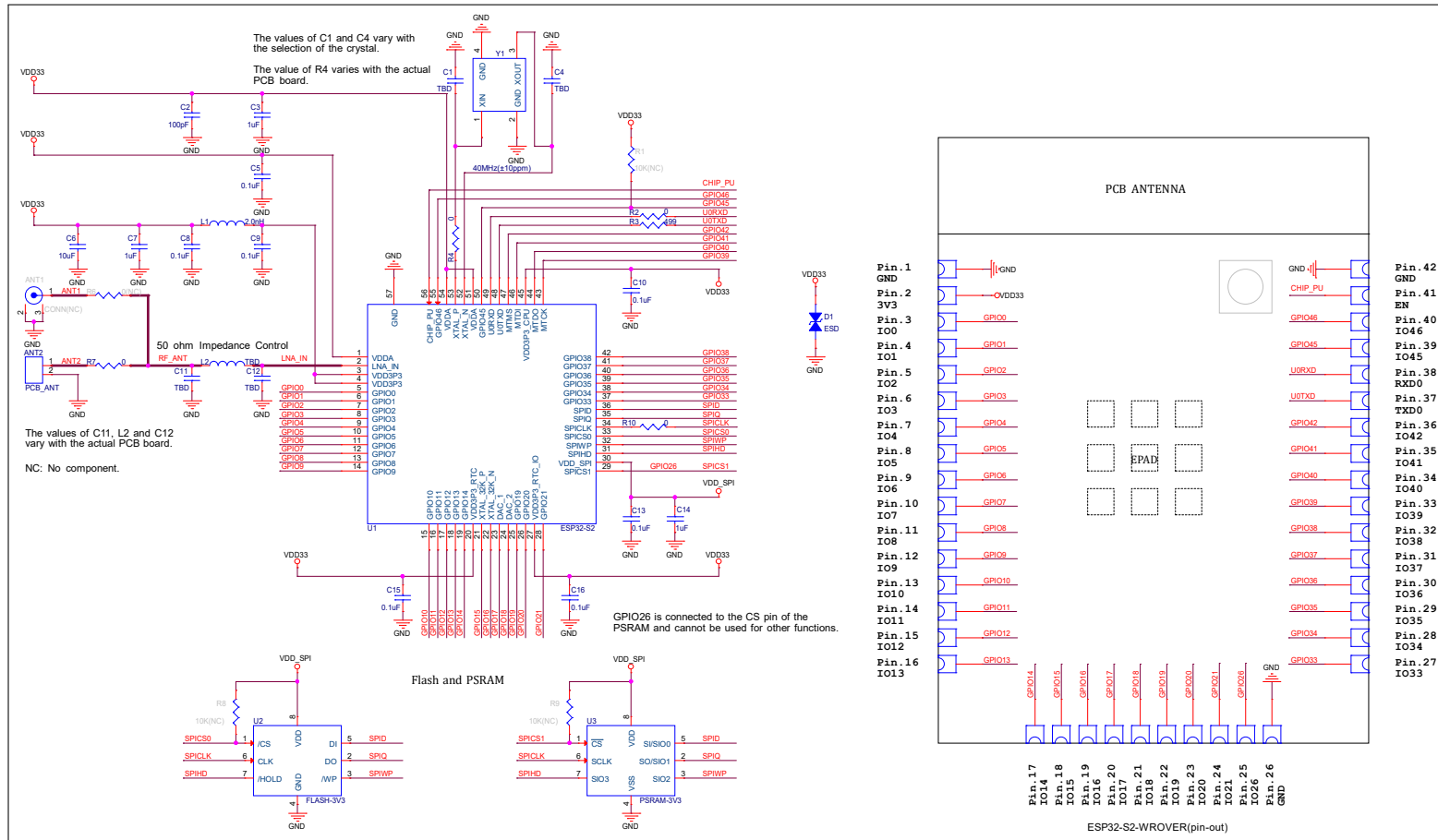
Figure 5: ESP32-S2-WROVER Schematics
