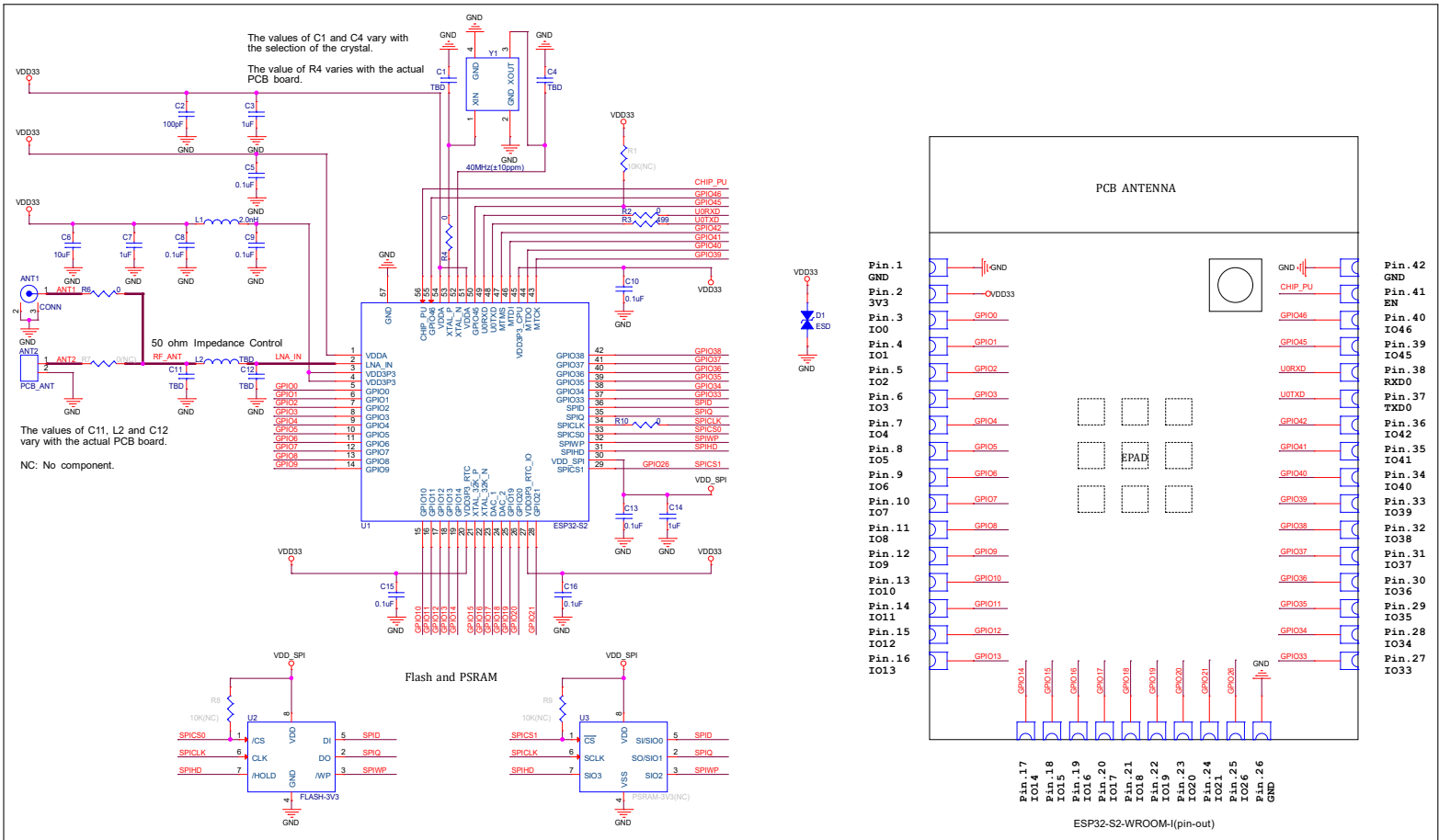
Figure 6: ESP32-S2-WROOM-I Schematics
