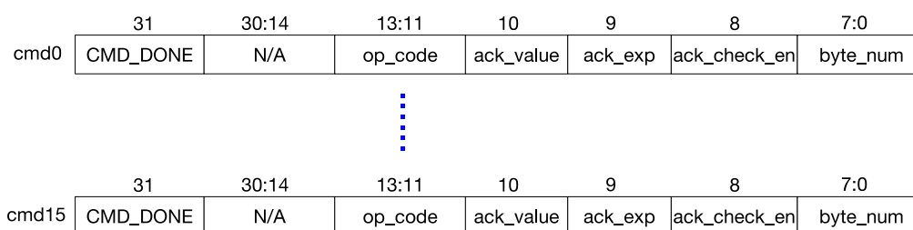
Figure 25-3. Structure of I2C Command Register
