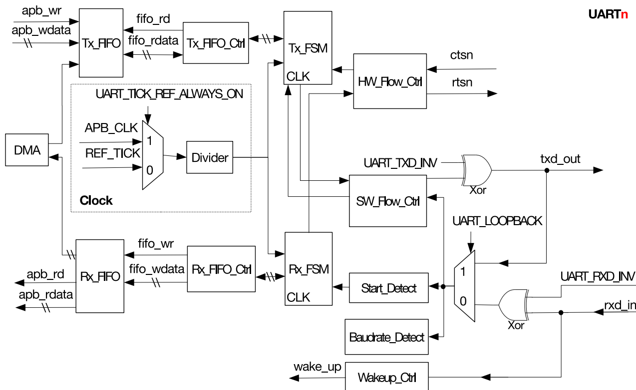
Figure 23-1. UART Structure
