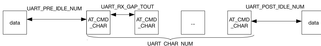
Figure 23-6. AT_CMD Character Structure
