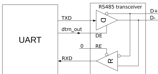
Figure 23-7. Driver Control Diagram in RS485 Mode
