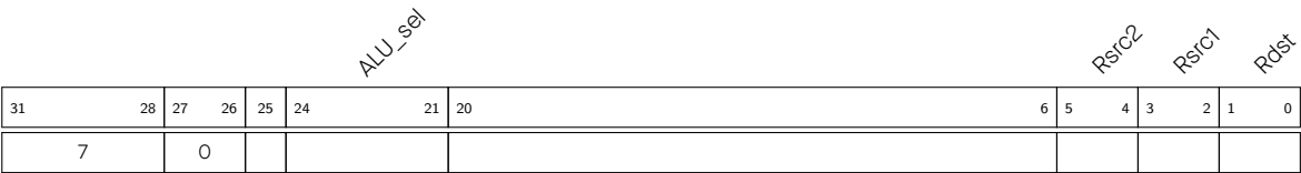
Figure 1-7. Instruction Type — ALU for Operations Among Registers
