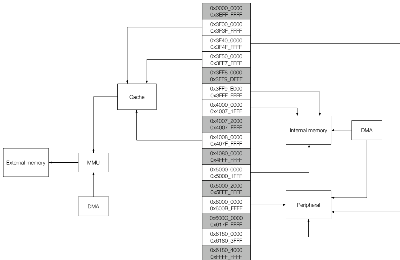
Figure 3-1. System Structure and Address Mapping
