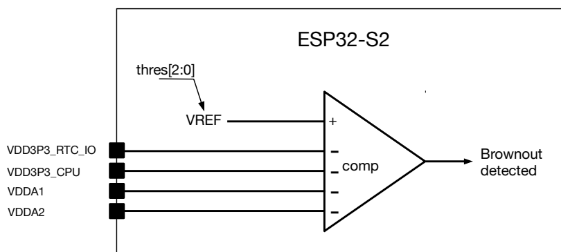
Figure 9-8. Brown-out detector
