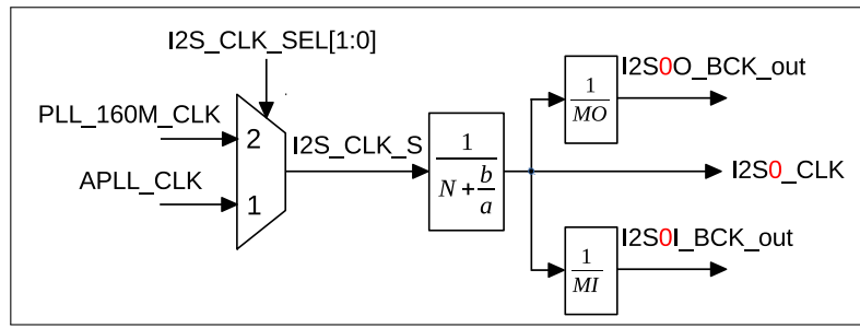
Figure 26-5. I2S Clock
