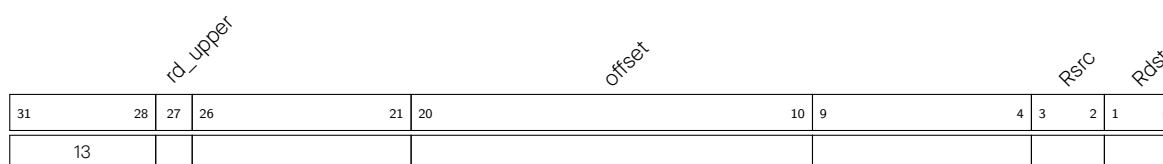
Figure 1-15. Instruction Type - LD
