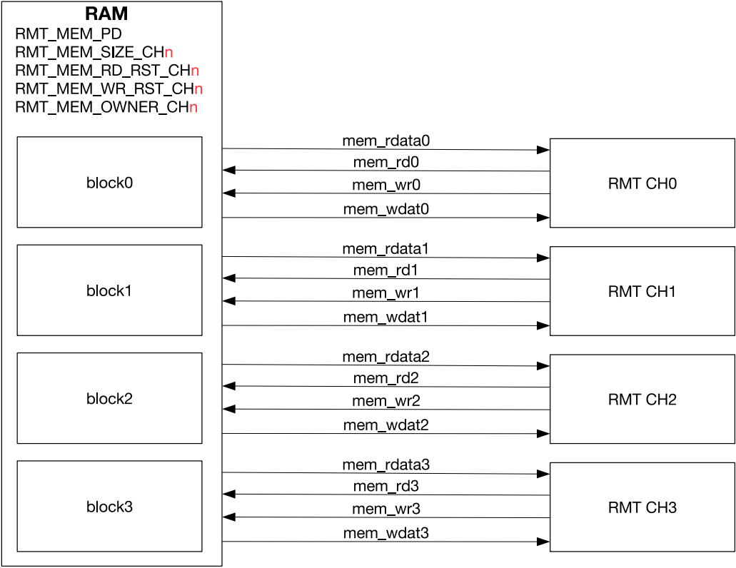
Figure 31-2. RMT Channels
