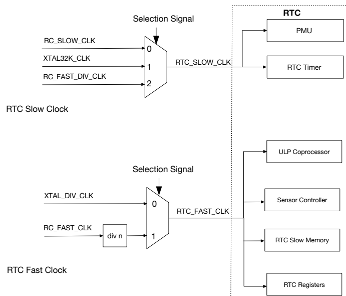
Figure 9-3. RTC_FAST_CLK and RTC_SLOW_CLK
