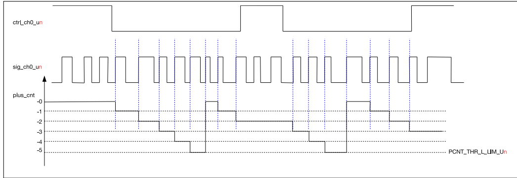
Figure 27-4. Channel 0 Down Counting Diagram
