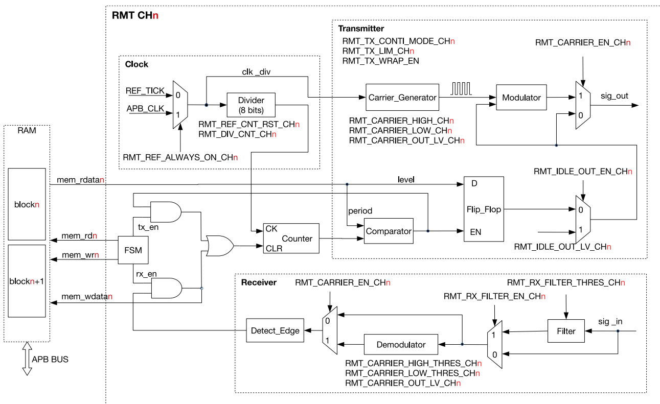
Figure 31-1. RMT Architecture
