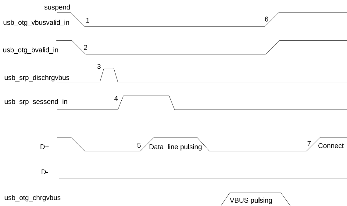
Figure 28-8. B-Device SRP
