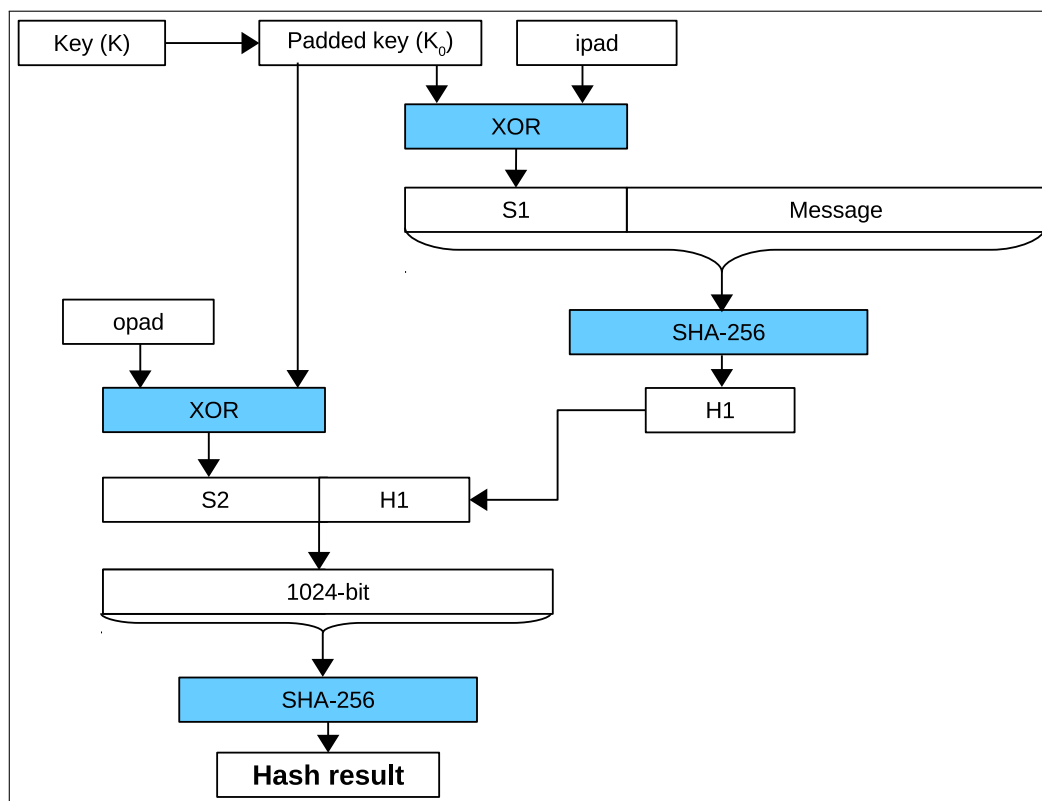
Figure 19-2. HMAC Structure Schematic Diagram
