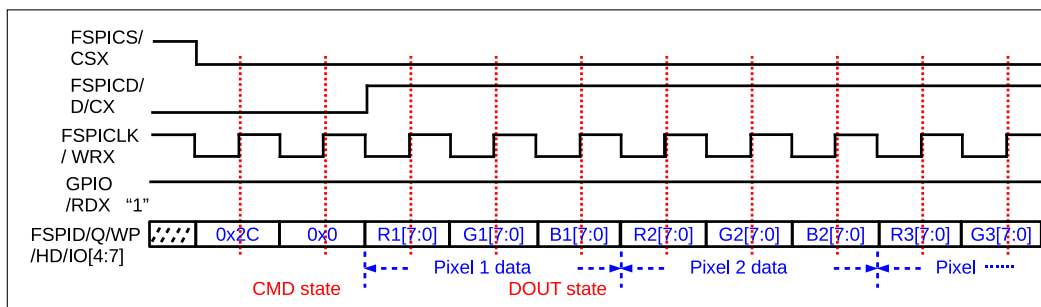
Figure 24-8. Write Command Sequence to an 8-bit LCD Driver
