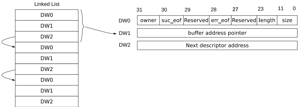
Figure 2-3. Structure of a Linked List
