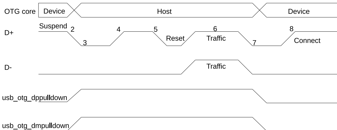
Figure 28-10. B-Device HNP
