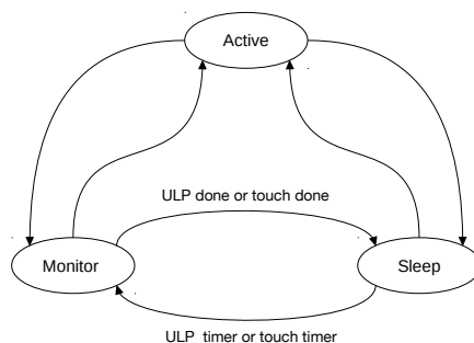
Figure 9-9. RTC States Transition
