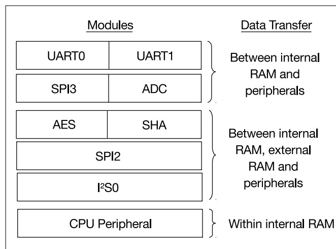
Figure 2-1. Modules with DMA and Supported Data Transfers
