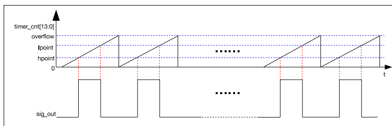
Figure 30-4. LED_PWM Output Signal Diagram
