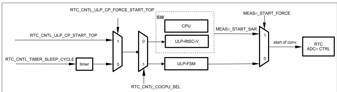
Figure 32-3. RTC SAR ADC Outline
