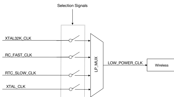
Figure 9-4. Low-Power Clocks for RTC Power Domains
