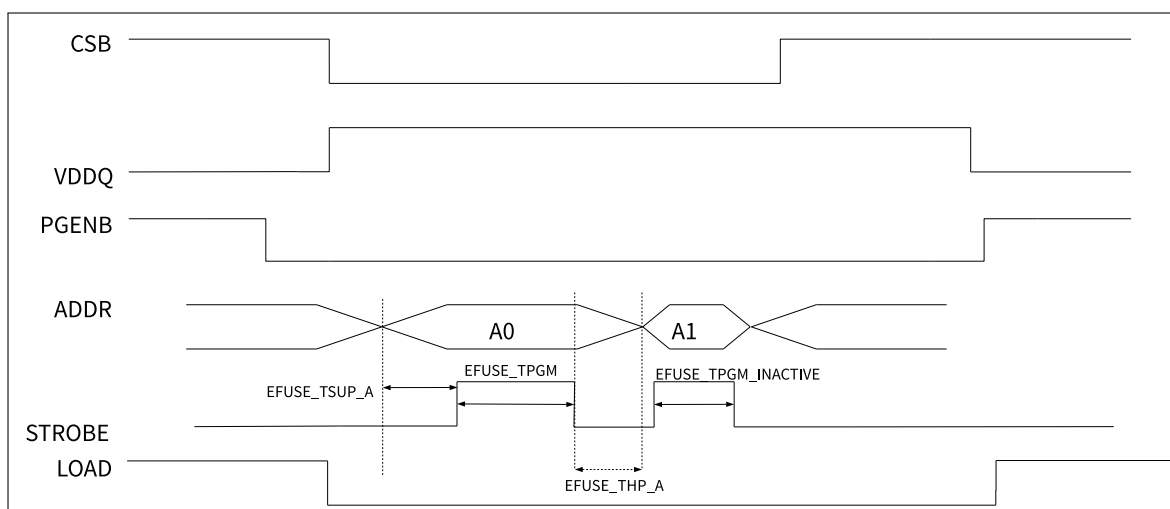
Figure 4-3. eFuse-Programming Timing Diagram
