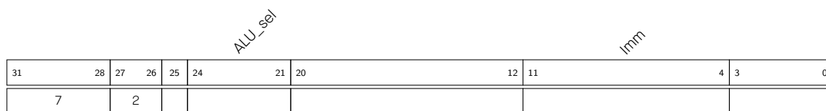
Figure 1-9. Instruction Type — ALU for Operations with Stage Count Register
