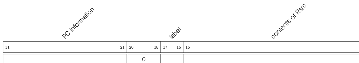
Figure 1-13. Data Structure of RTC_SLOW_MEM[Rdst + Offset]
