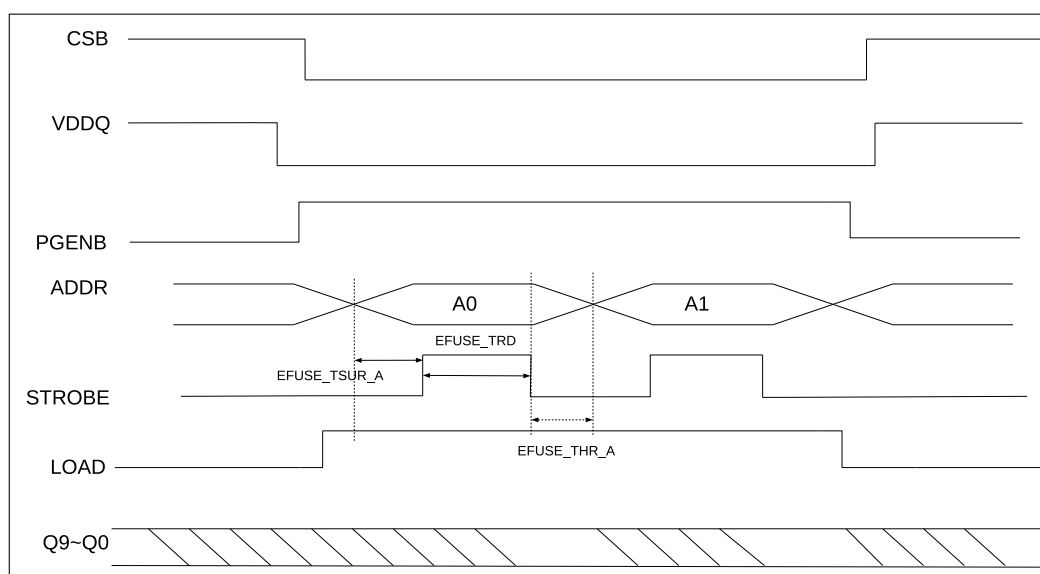
Figure 4-4. Timing Diagram for Reading eFuse
