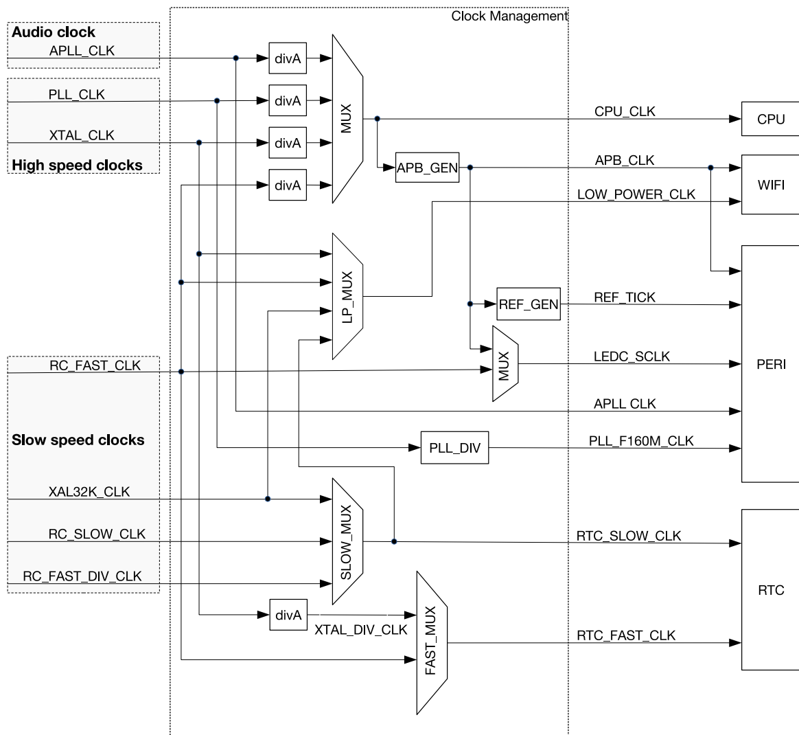
Figure 6-2. System Clock
