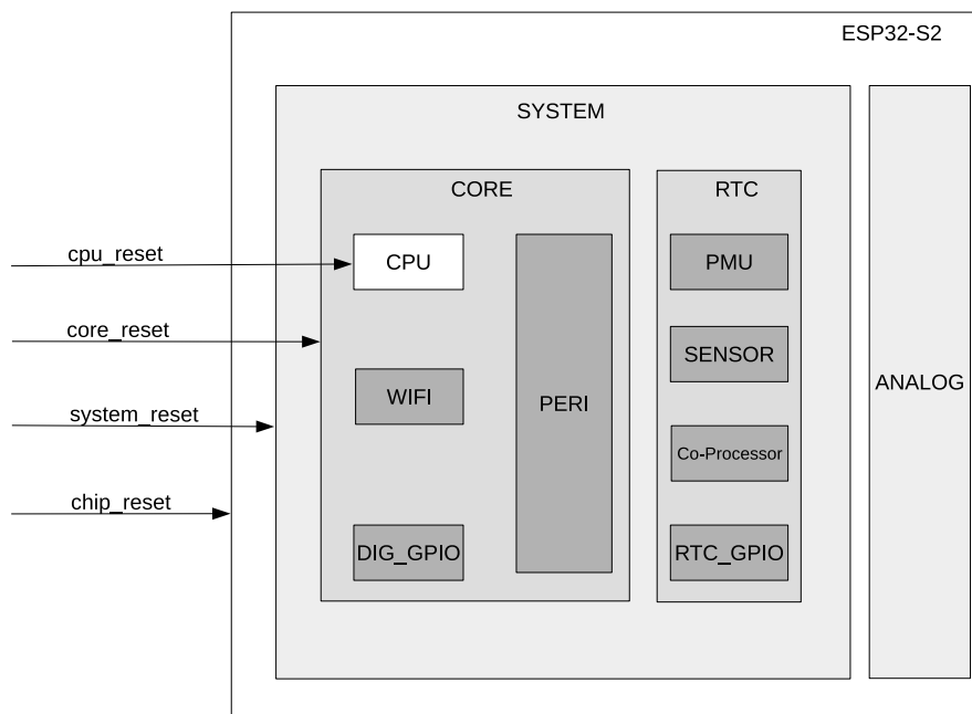
Figure 6-1. Reset Level
