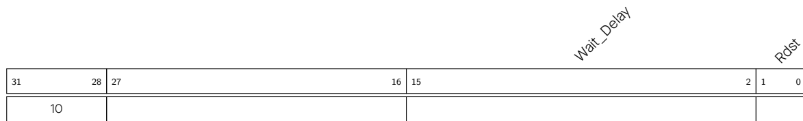
Figure 1-22. Instruction Type - TSENS
