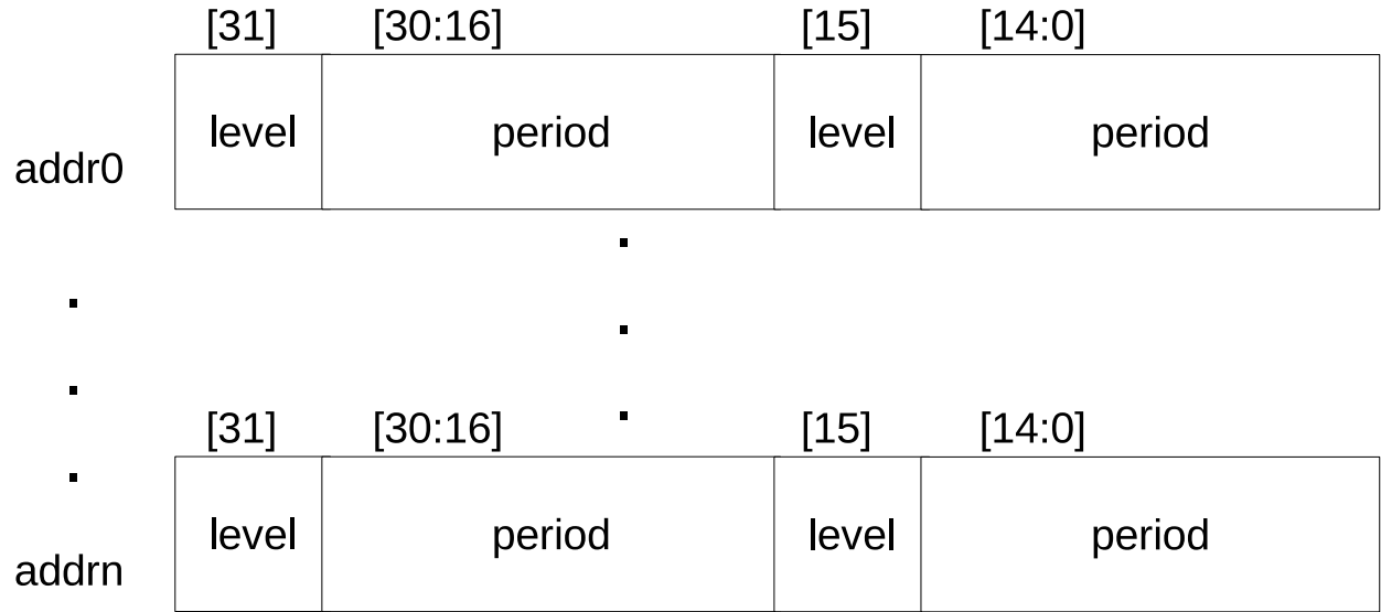
Figure 31-3. Format of Pulse Code in RAM
