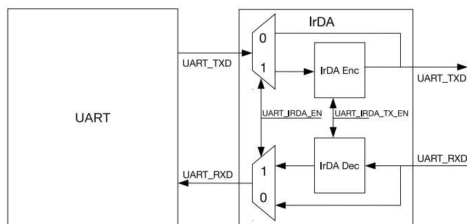
Figure 23-9. IrDA Encoding and Decoding Diagram
