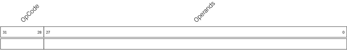
Figure 1-6. ULP-FSM Instruction Format
