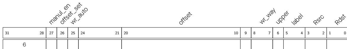
Figure 1-10. Instruction Type - ST
