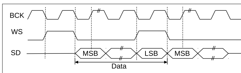
Figure 26-4. PCM Standard
