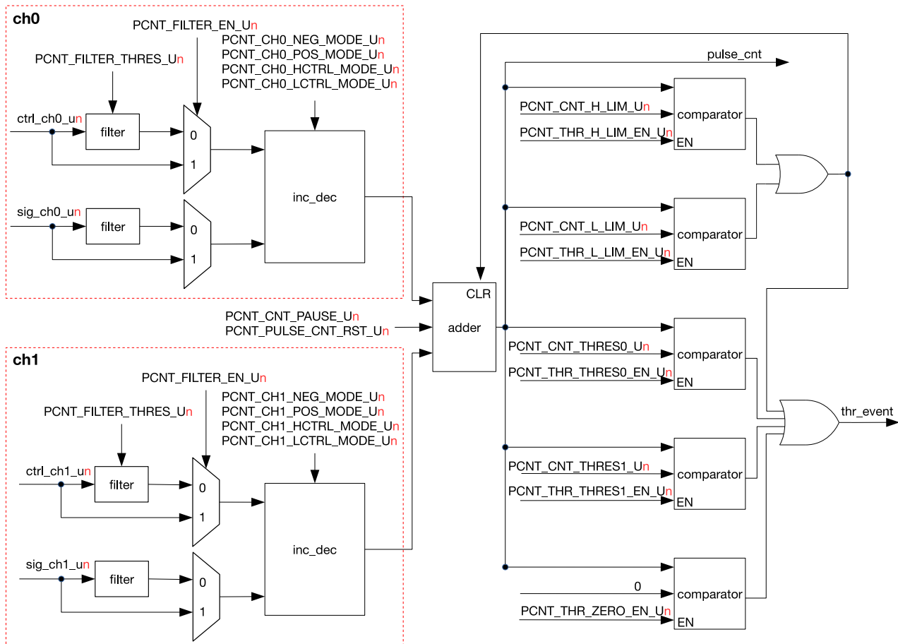
Figure 27-2. PCNT Unit Architecture
