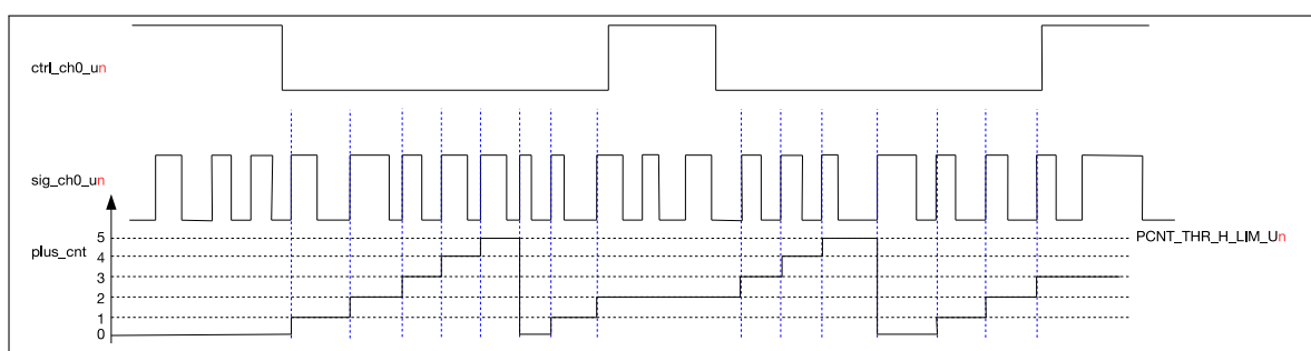
Figure 27-3. Channel 0 Up Counting Diagram
