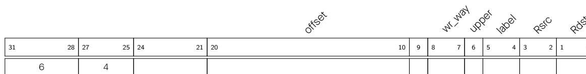
Figure 1-14. Instruction Type - Data Storage in Manual Storage Mode
