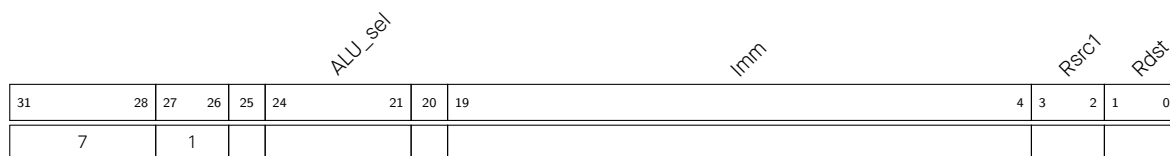
Figure 1-8. Instruction Type — ALU for Operations with Immediate Value
