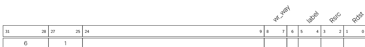
Figure 1-12. Instruction Type - Data Storage in Automatic Storage Mode (ST-AUTO-DATA)
