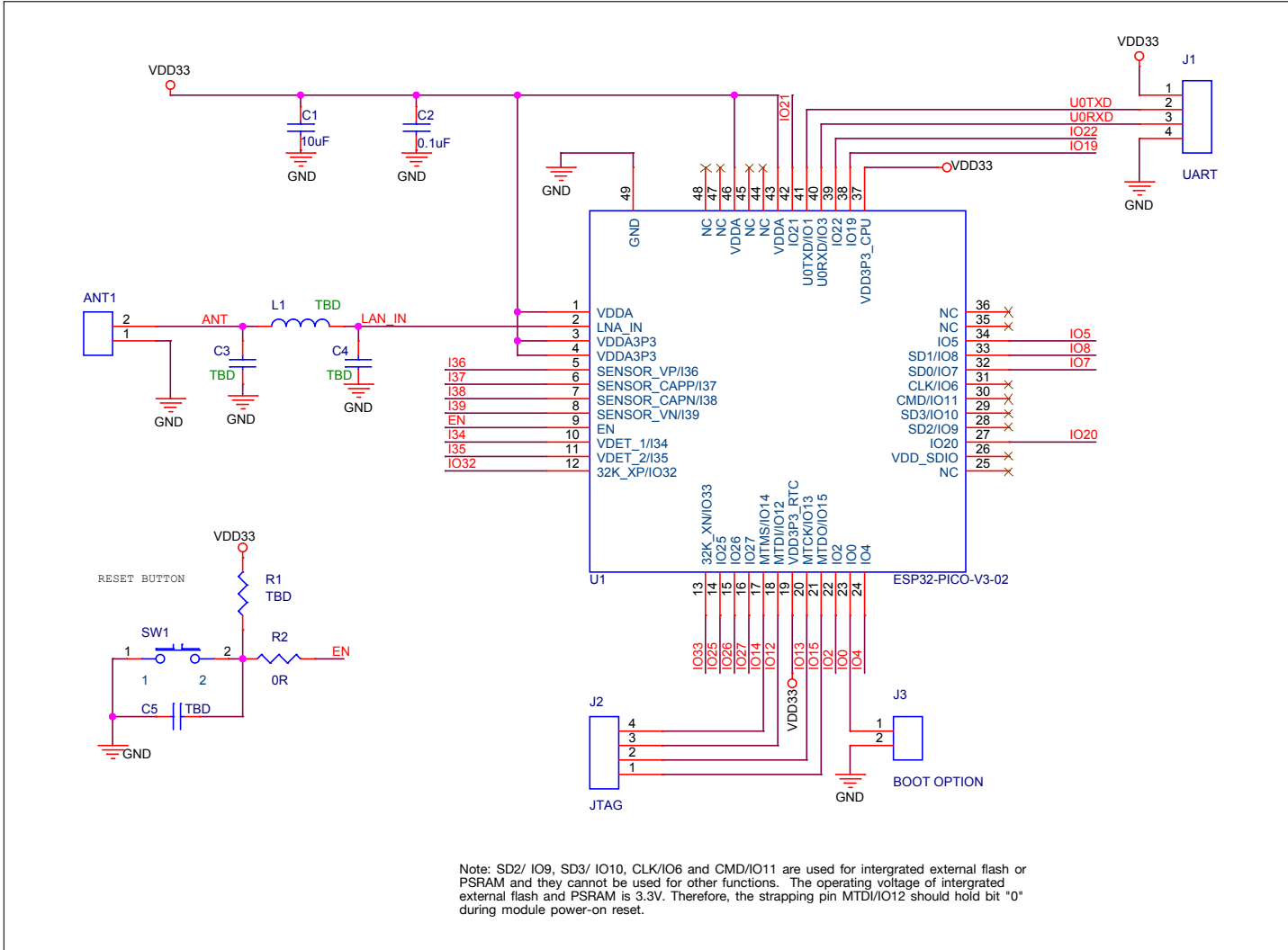
Figure 12: ESP32-PICO-V3-02 Peripheral Schematics
