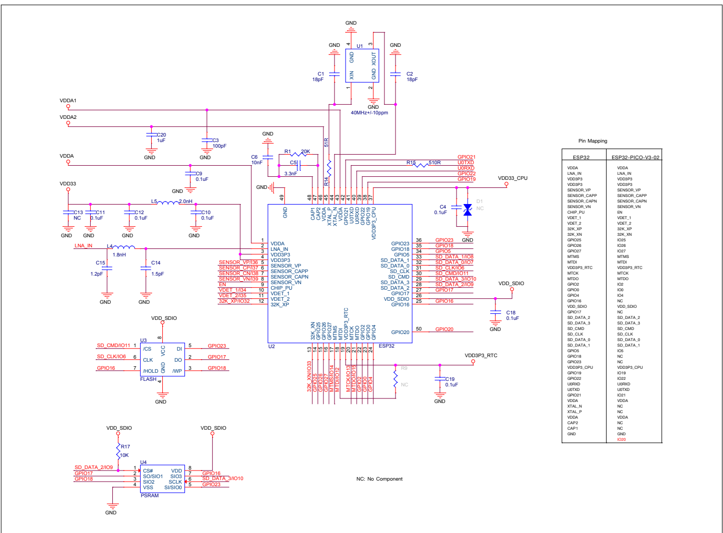
Figure 9: ESP32-PICO-V3-02 Schematics
