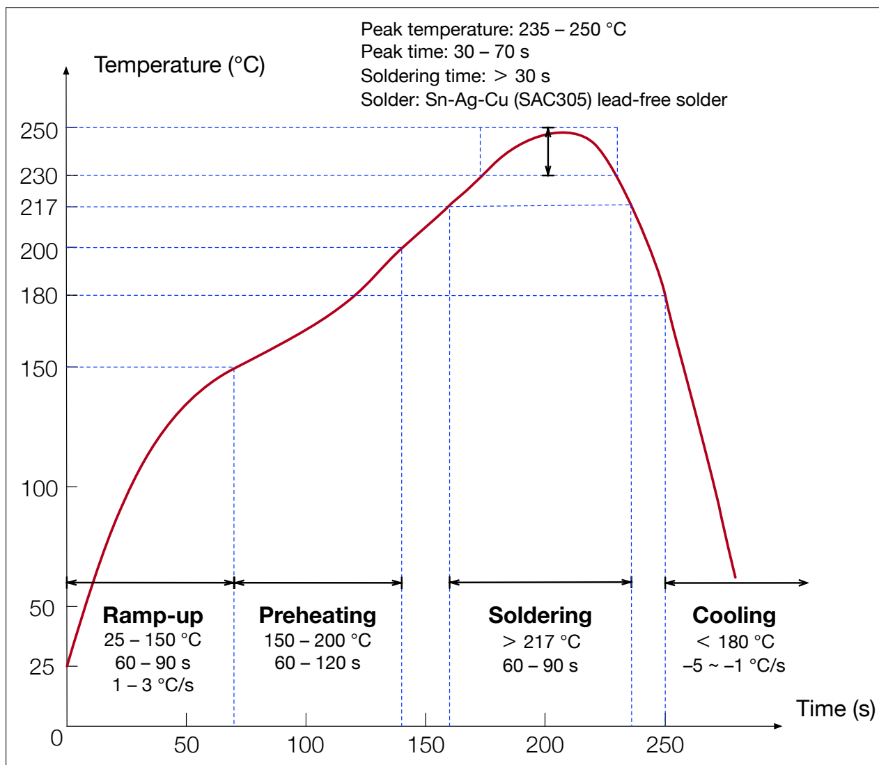
Figure 13: Reflow Profile
