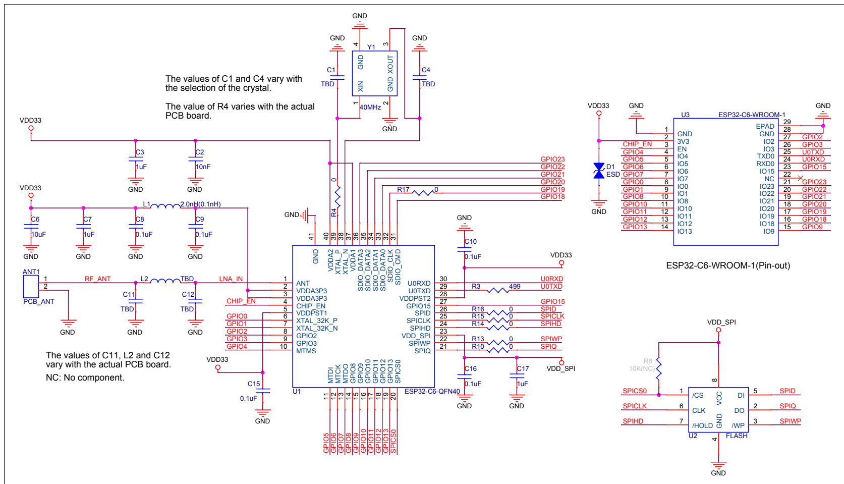
Figure 5: ESP32-C6-WROOM-1 Schematics
