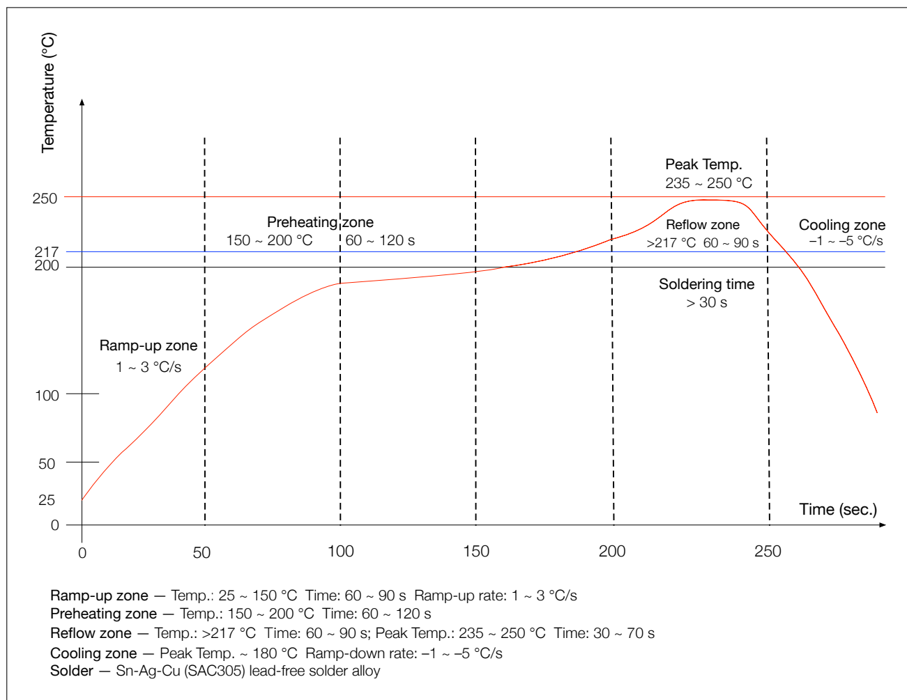
Figure 4: Reflow Profile
