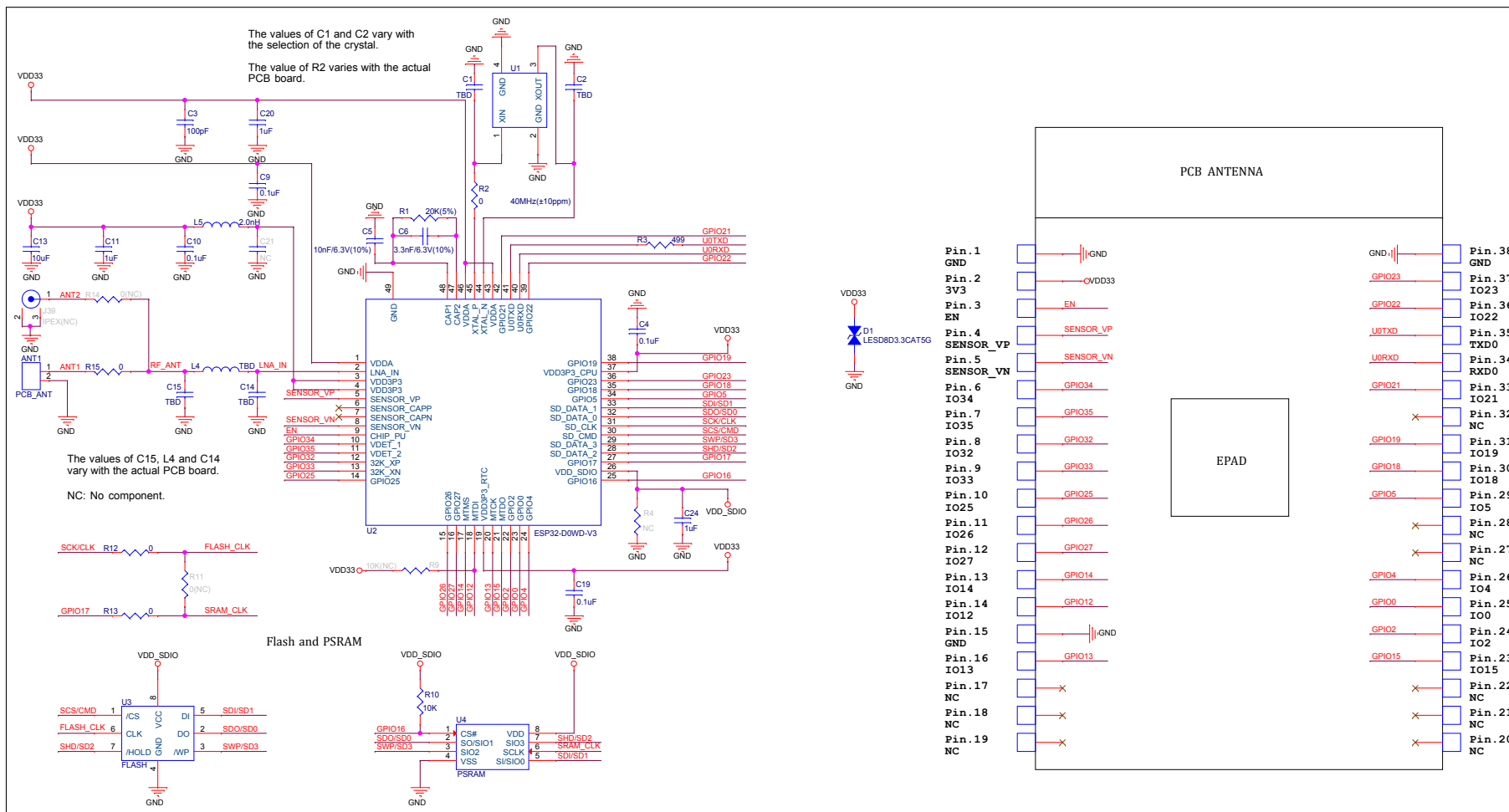
Figure 5: Schematics of ESP32-WROVER-E
