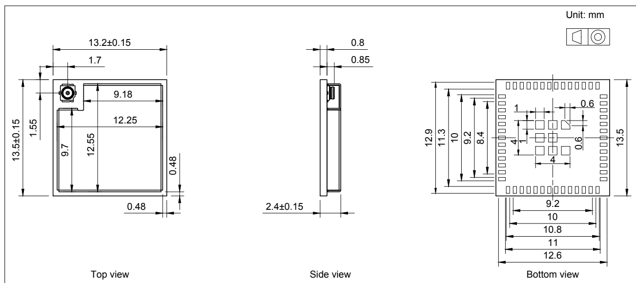
Figure 9: ESP32-MINI-1U Physical Dimensions
