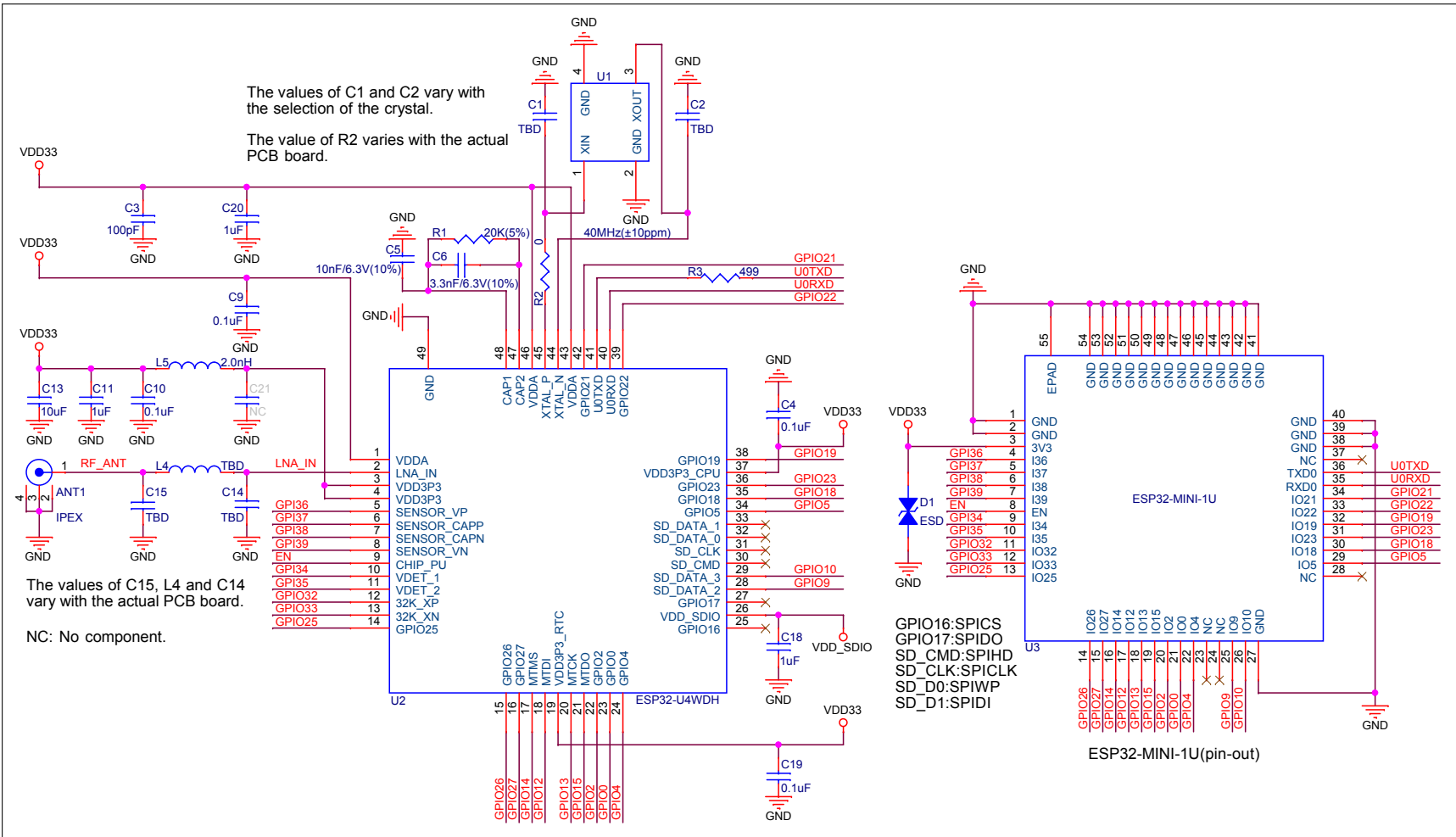
Figure 6: ESP32-MINI-1U Schematics
