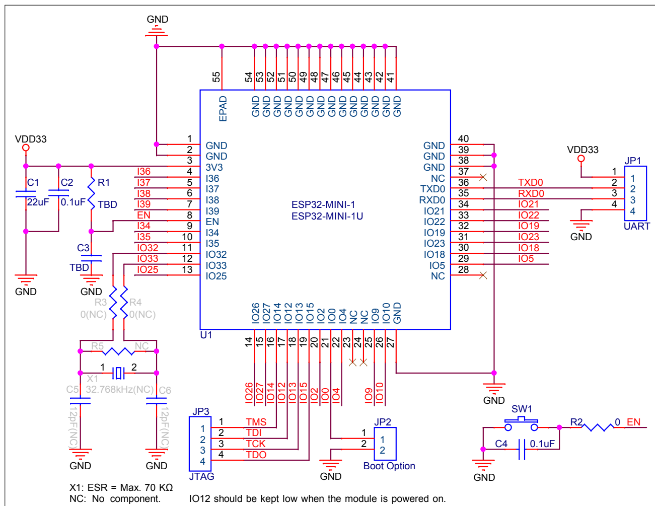
Figure 7: Peripheral Schematics
