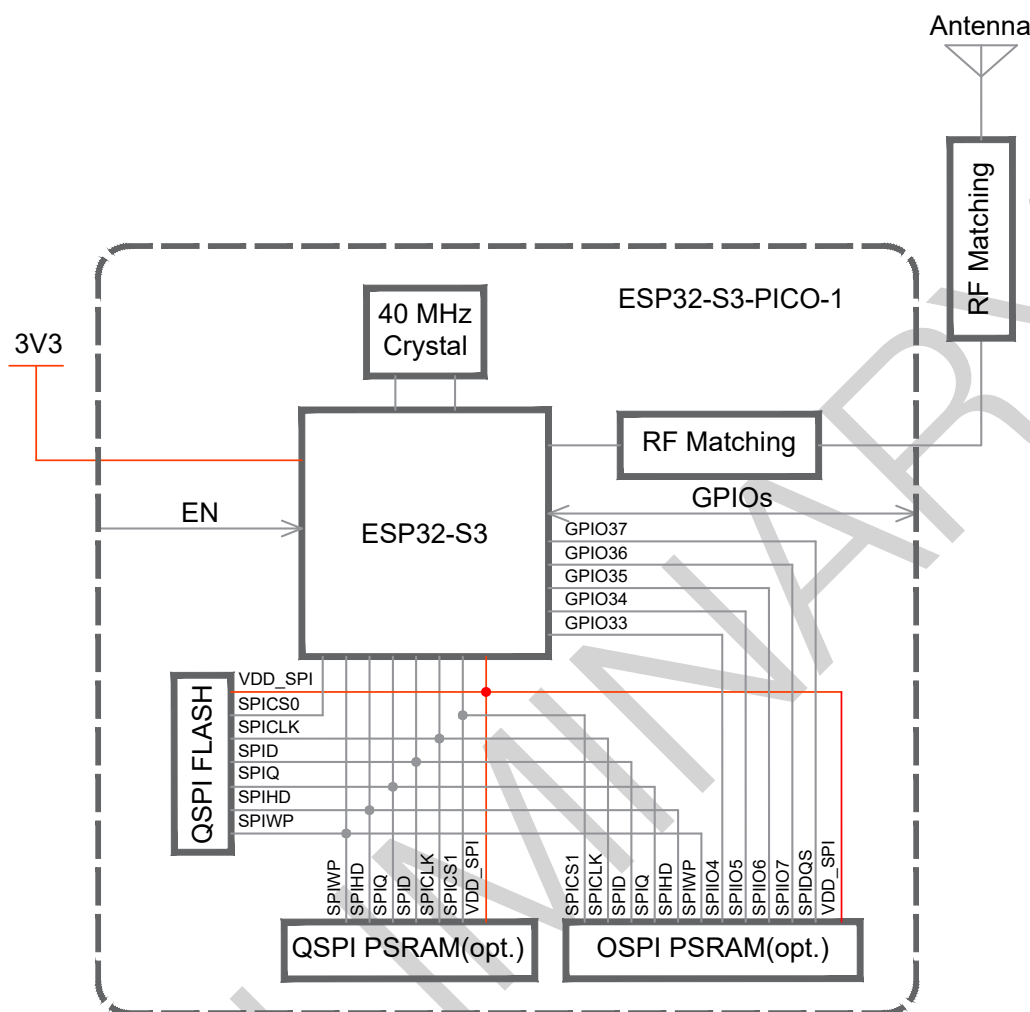
Figure 0-1. ESP32-S3-PICO-1 Block Diagram
