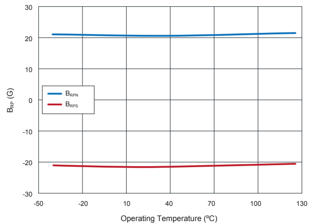
14.7 RR122-1B12-511 / 512 B_{RPN} (Blue) and B_{RPS} (Red) vs. Operating Temperature at V_{DD}=3.0 V
