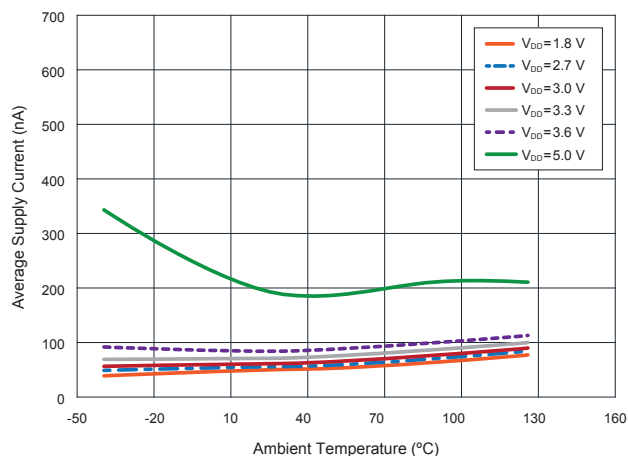
14.2 RR122-1B12-511 / 512 Average Supply Current vs. Temperature vs. Supply Voltage
