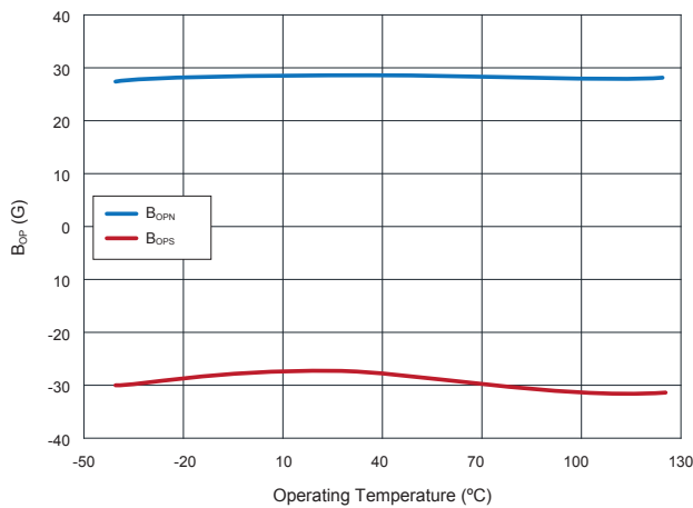
14.6 RR122-1B12-511 / 512 B_{OPN} (Blue) and B_{OPS} (Red) vs. Operating Temperature at V_{DD}=3.0 V
