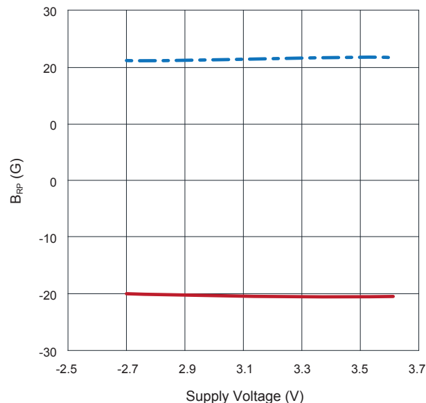
7.6 B_{RPN} (Blue) and B_{RPS} (Red) vs. Supply Voltage at +25^\circ\text{C}
