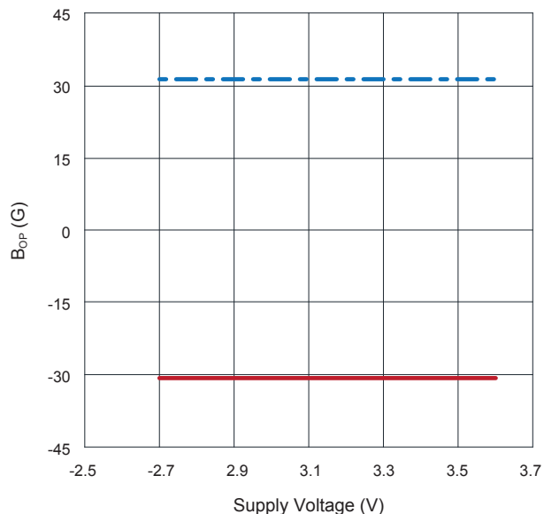
7.5 B_{OPN} (Blue) and B_{OPS} (Red) vs. Supply Voltage at +25^\circ\text{C}
