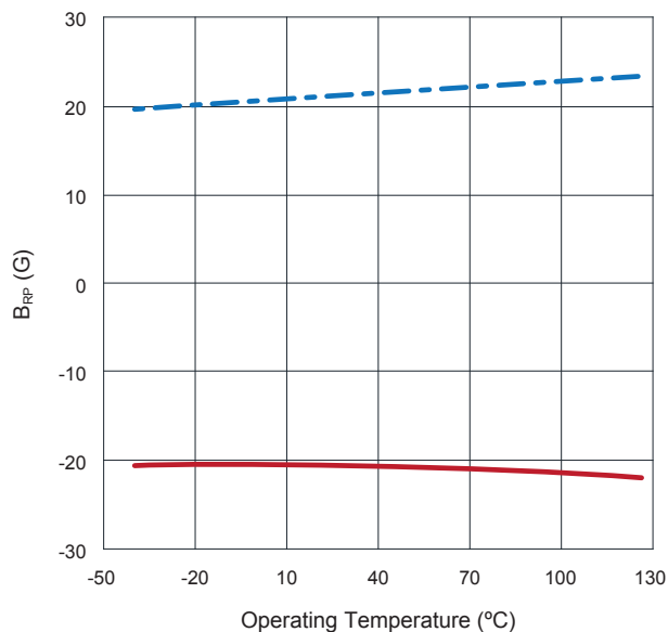
7.8 B_{RPN} (Blue) and B_{RPS} (Red) vs. Operating Temperature at V_{DD}=3.0\text{ V}
