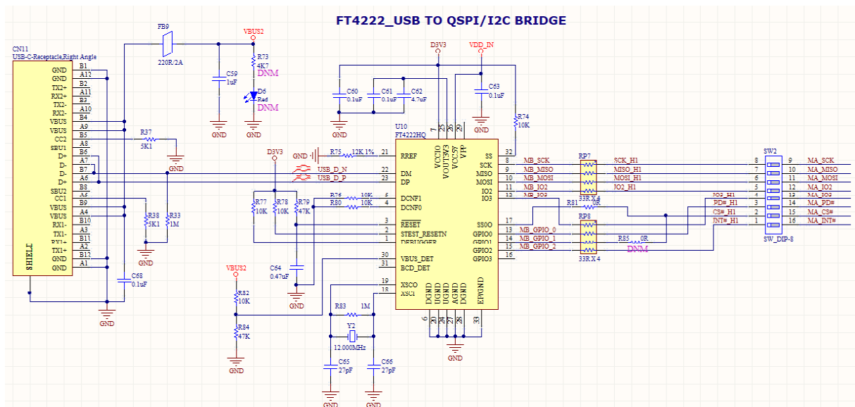
Figure 4-2 - FT4222 USB Bridge Circuit
