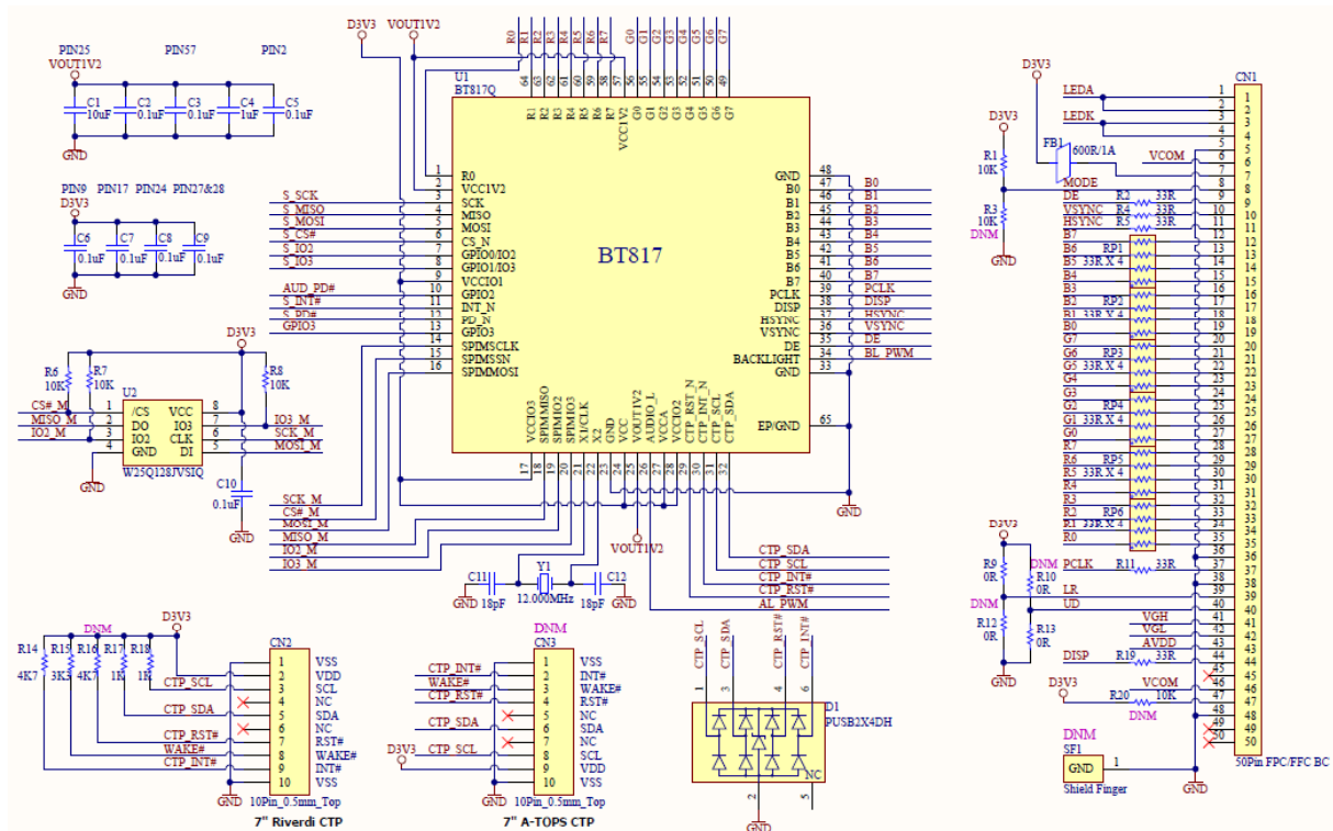
Figure 4-1 - BT817 IC and RGB Connector
