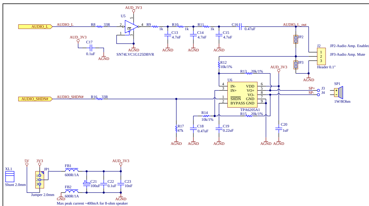
Figure 4-3 – Audio Circuit
