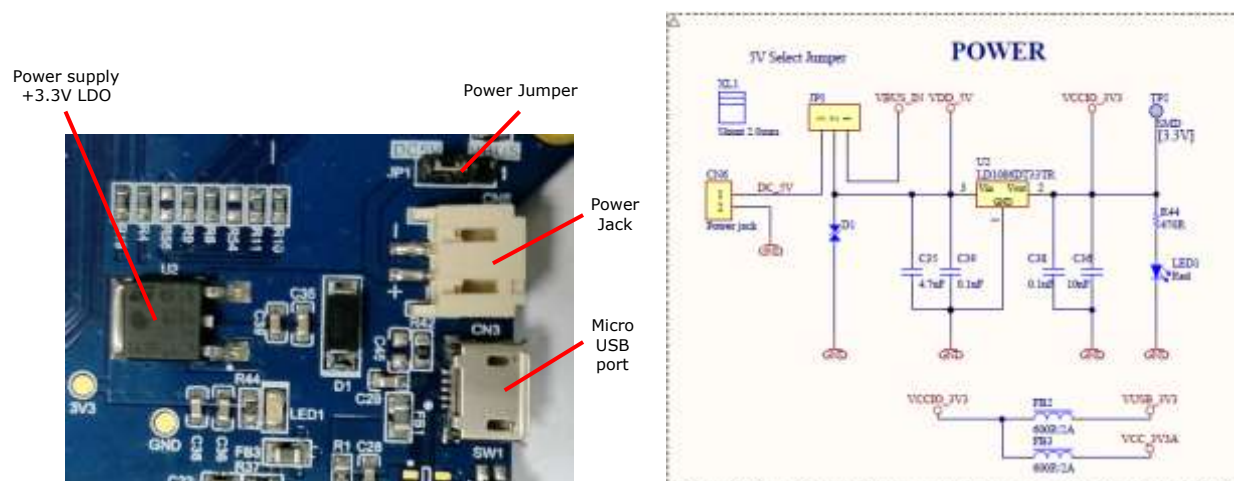
Figure 4-2– Power supply
