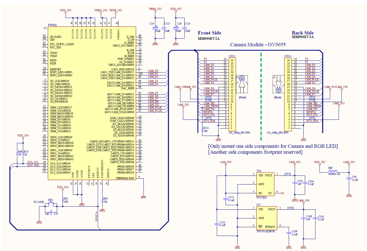
Figure 4-12 – Camera connector
