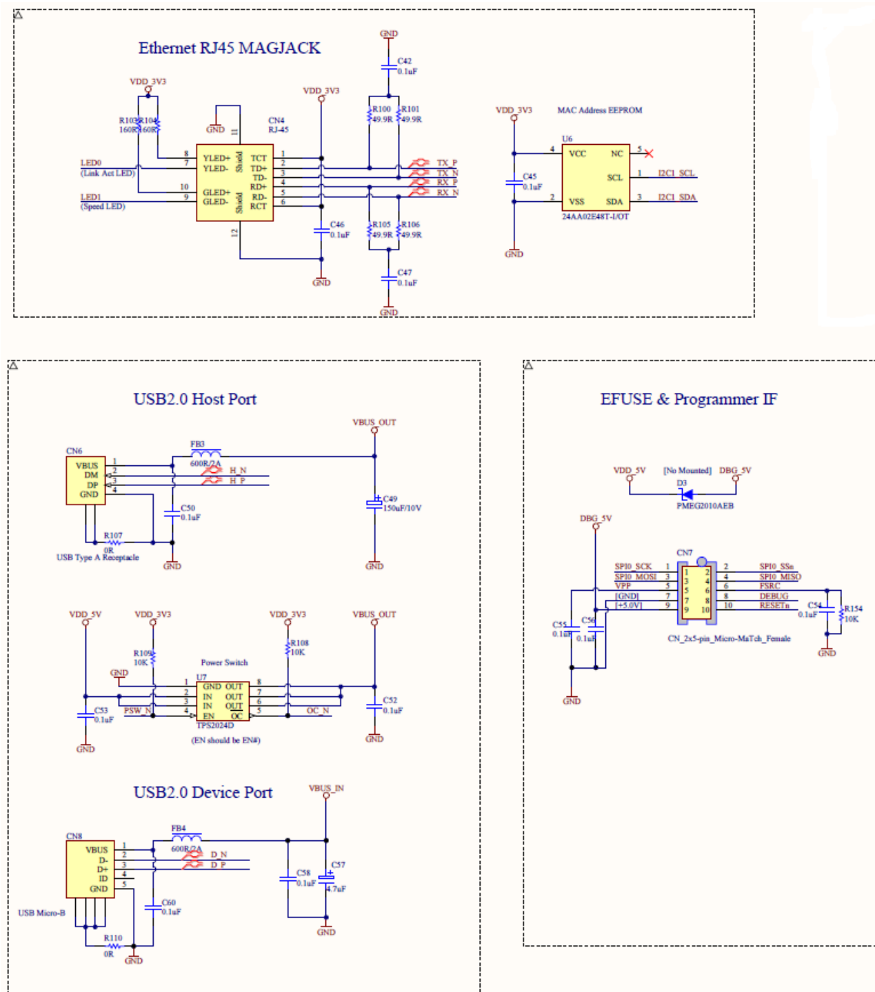
Figure 5-3 – Sheet 2-FT900 Interfaces and Connectors(1)
