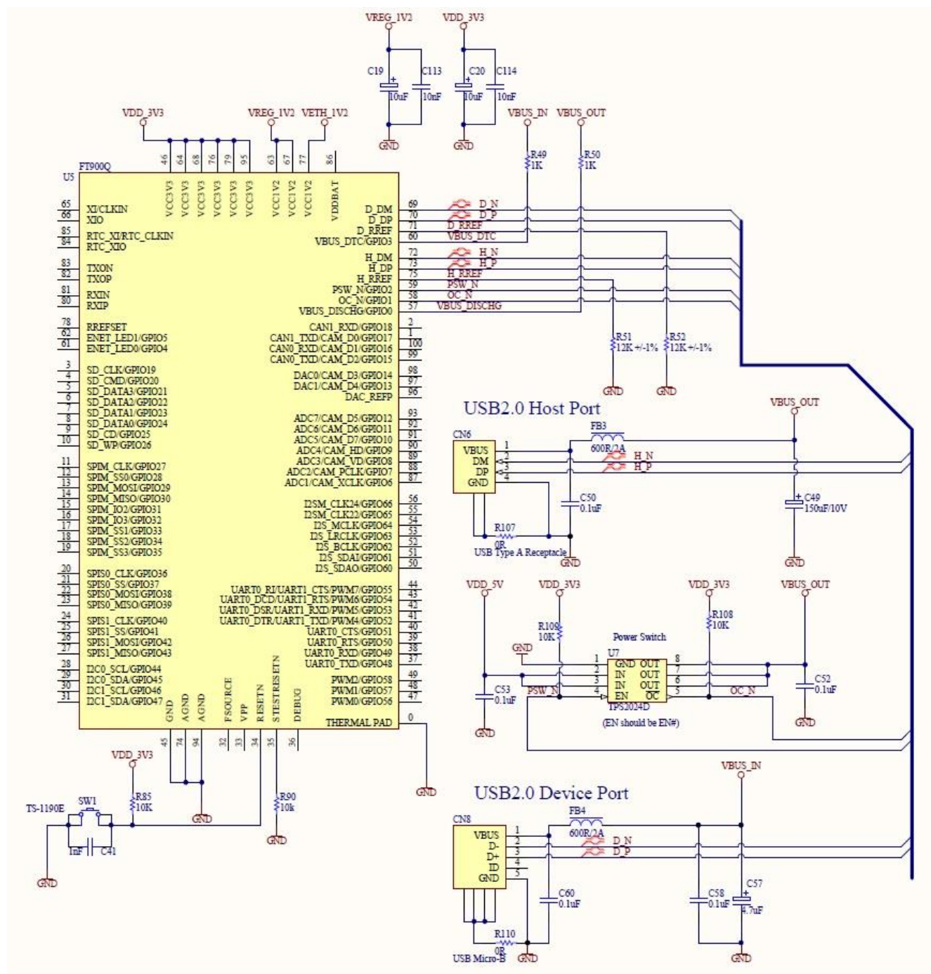
Figure 4-6 – USB Connectors
