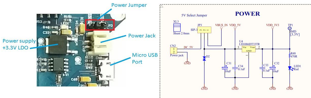
Figure 4-3 – Power supply
