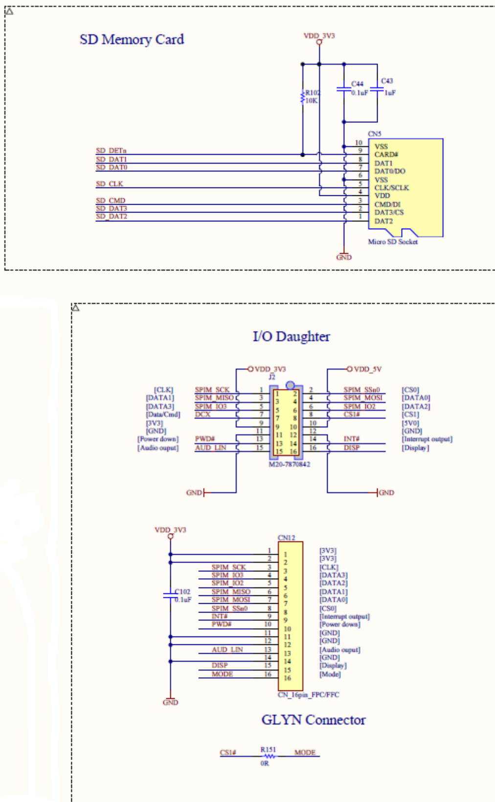
Figure 5-4 – Sheet 2-FT900 Interfaces and Connectors(1)
