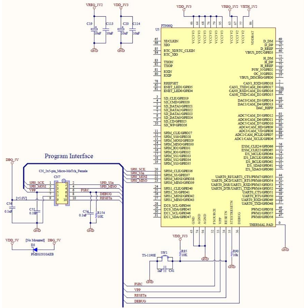
Figure 4-8 – Program Interface
