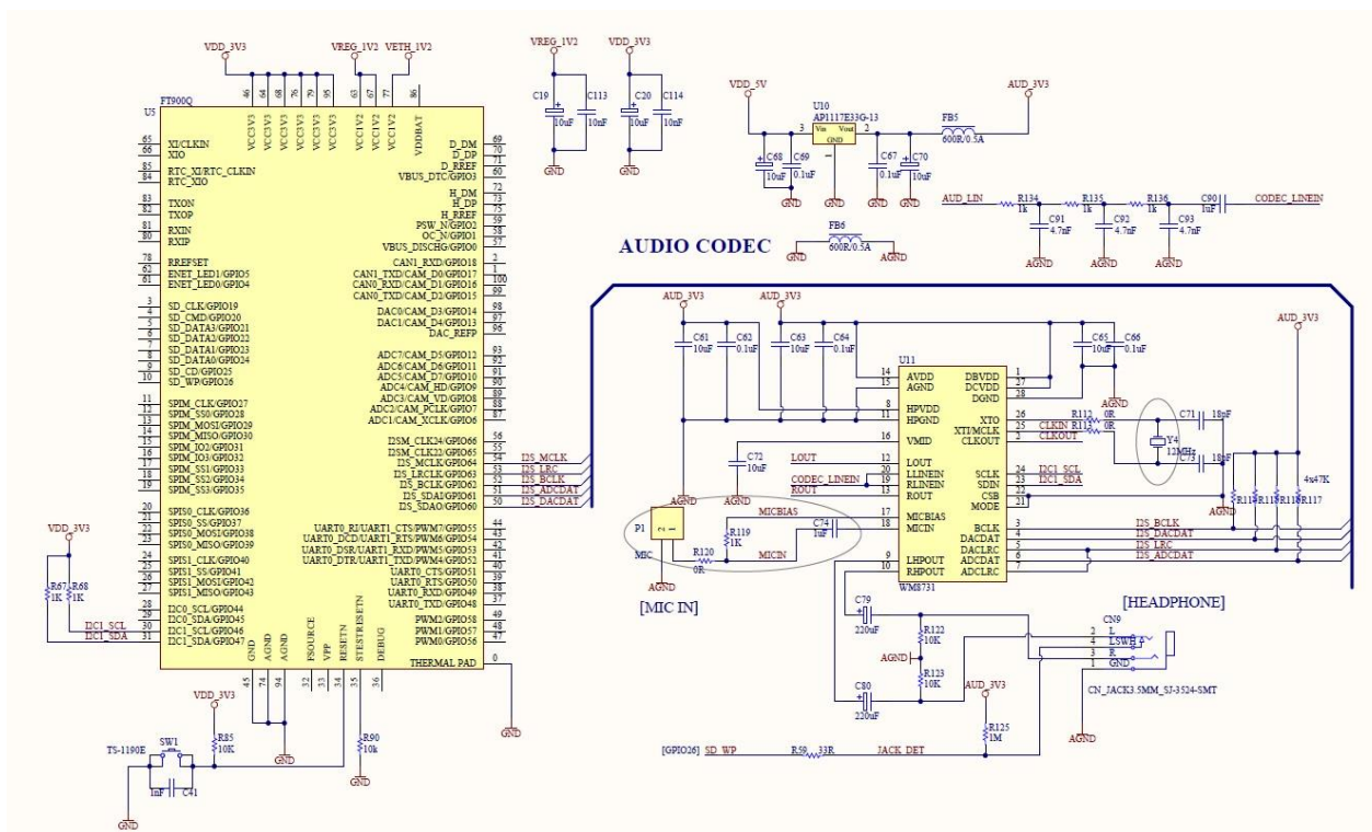
Figure 4-10 – Microphone Input
