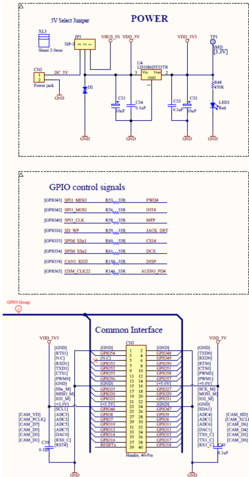
Figure 5-2 – Sheet 1-FT900 MCU(2)
