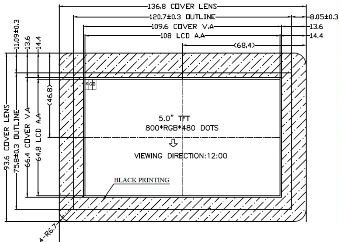
Figure 6-3 – Touch and Display Dimensions
