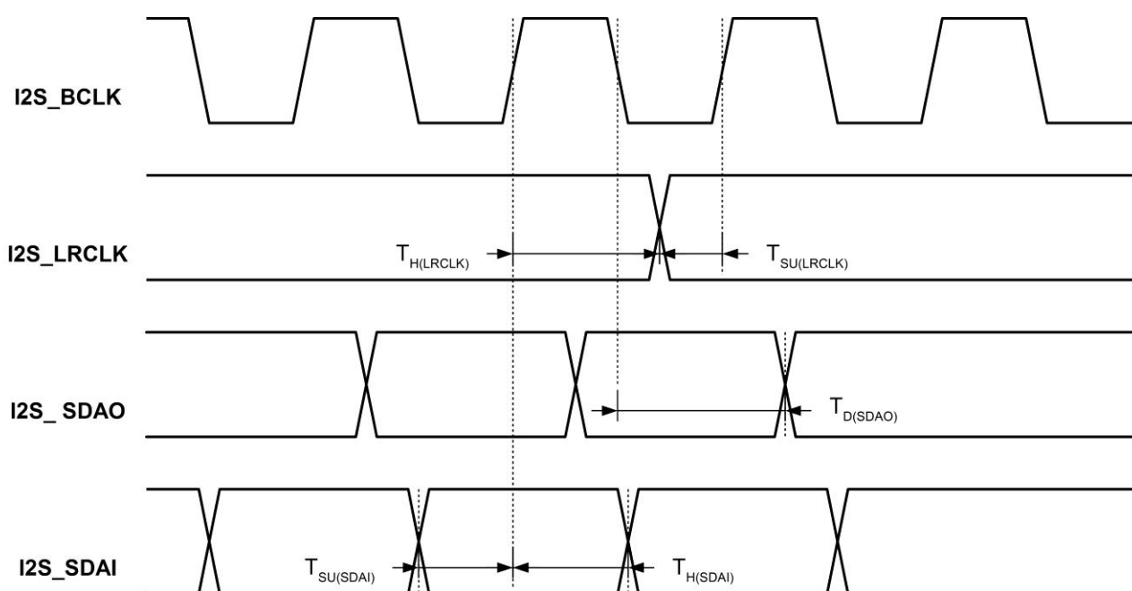
Figure 5-10 Definition of I 2 S Slave Timing
