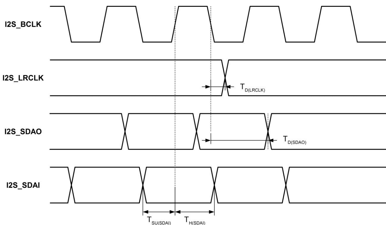
Figure 5-9 Definition of I 2 S Master Timing
