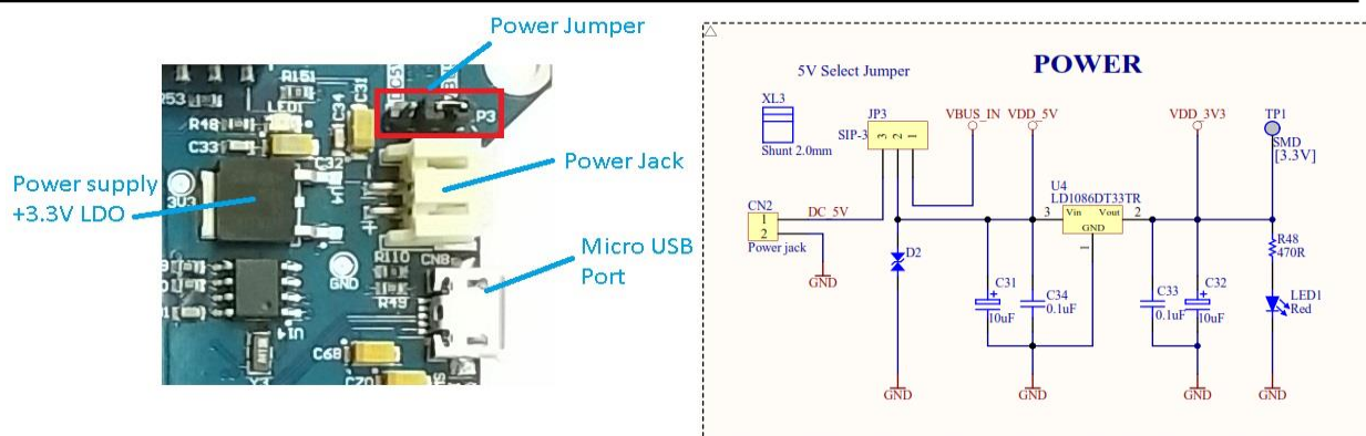
Figure 4-3 – Power supply
