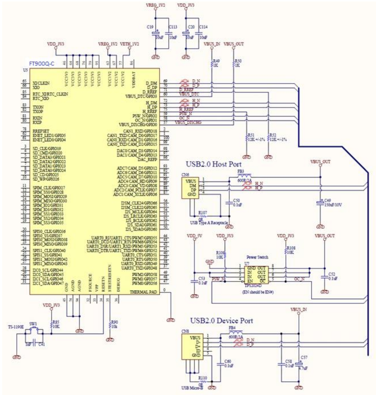
Figure 4-6 – USB Connectors
