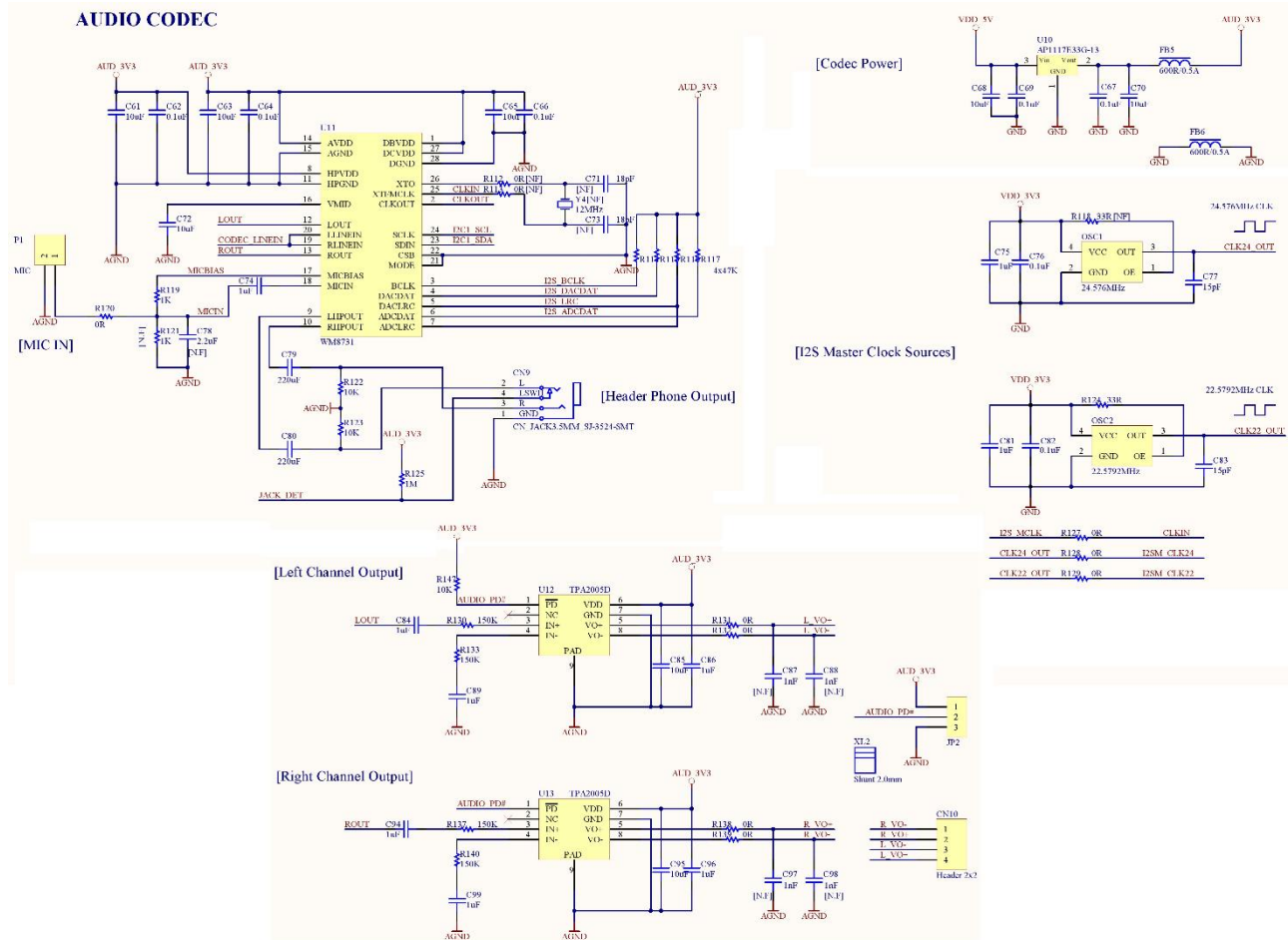
Figure 4-11 – Audio Output
