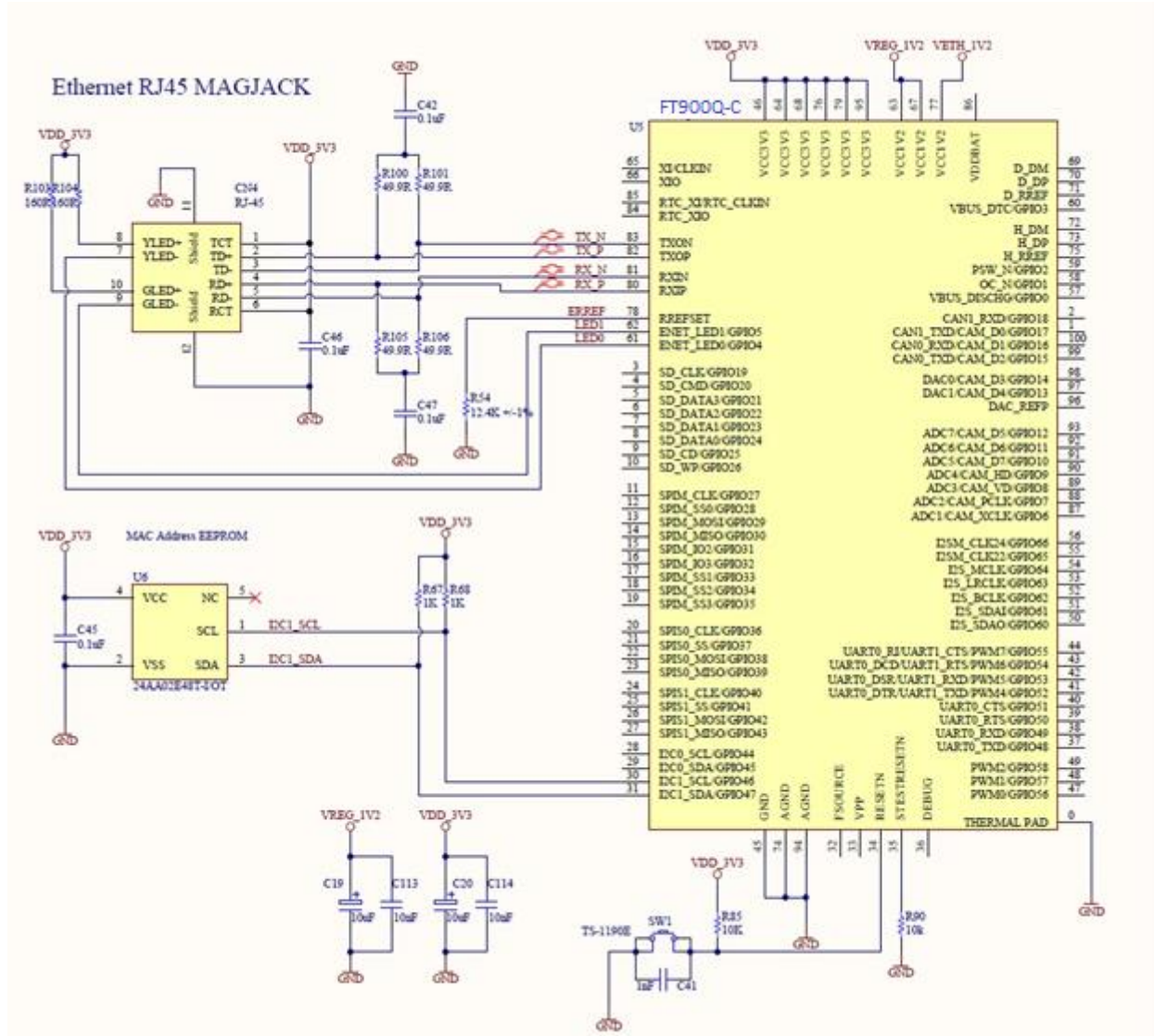
Figure 4-7 – Ethernet connector
