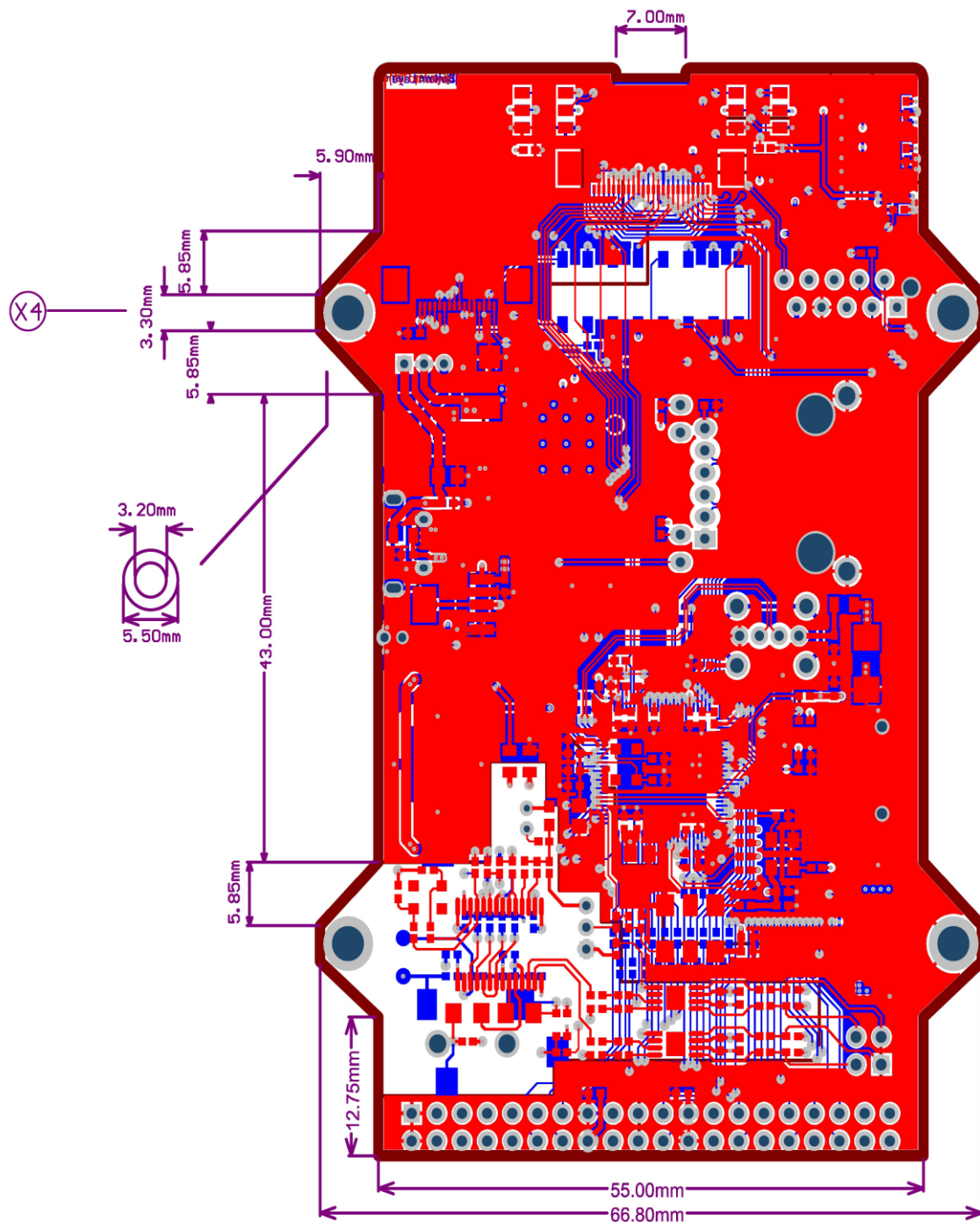
Figure 6-2 – MM900EV2B/3B PCB Dimensions
