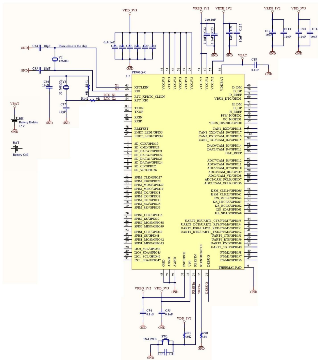
Figure 4-14 – RTC
