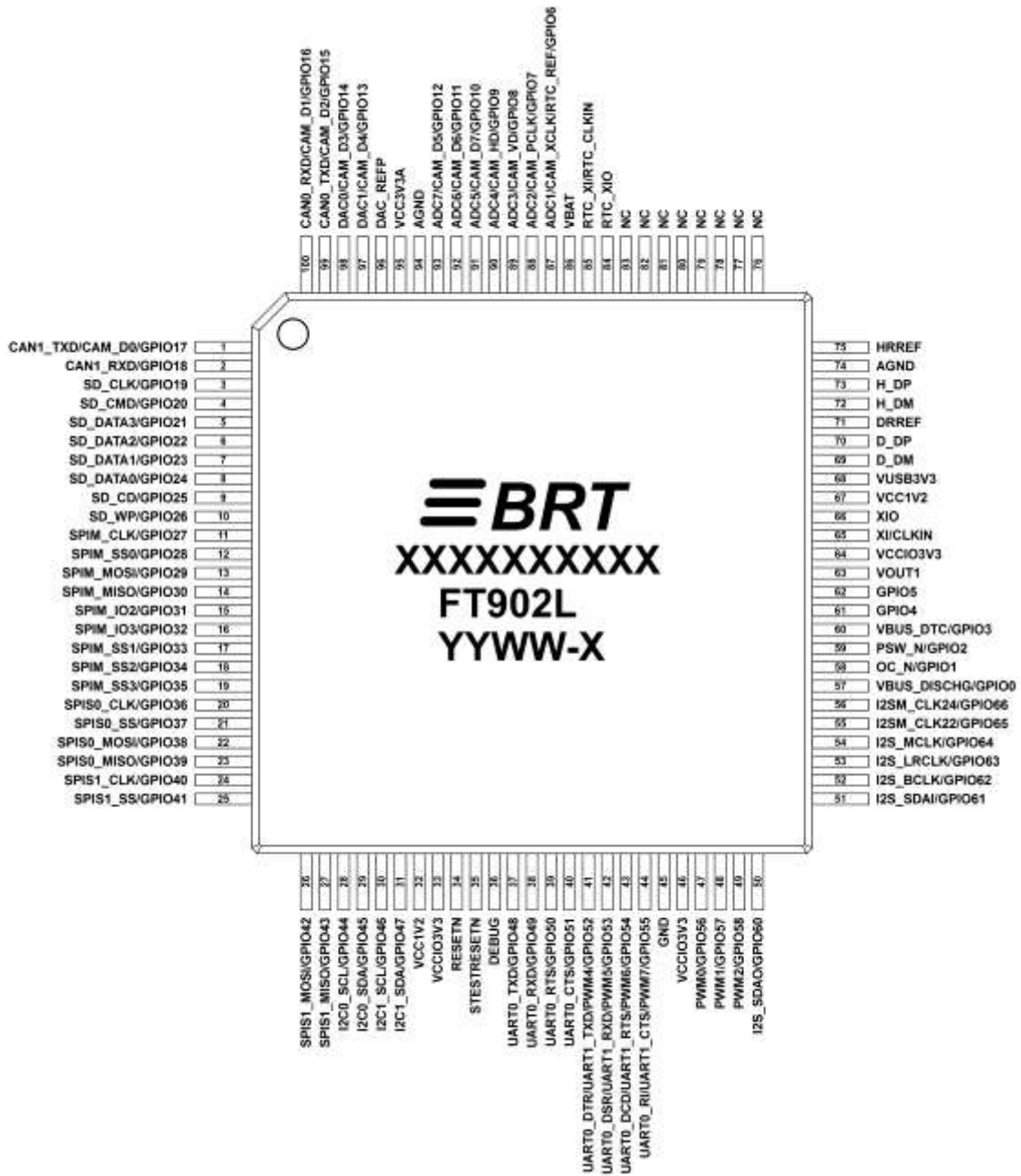
Figure 3-7 - Pin Configuration FT902L (top-down view)
