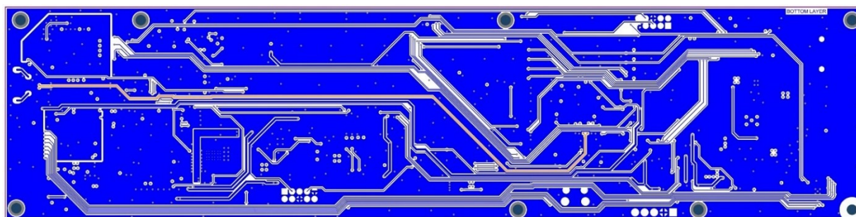
Figure 12 - Main PCB Bottom Layer
