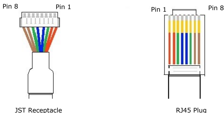
Figure 28 - JST8-RJ45 Cable Pin Orientation
