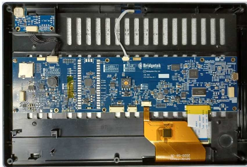
Figure 39 - Main PCBA and Speaker Board
