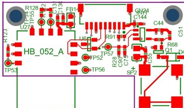
Figure 15 - Sound PCB Top Layer
