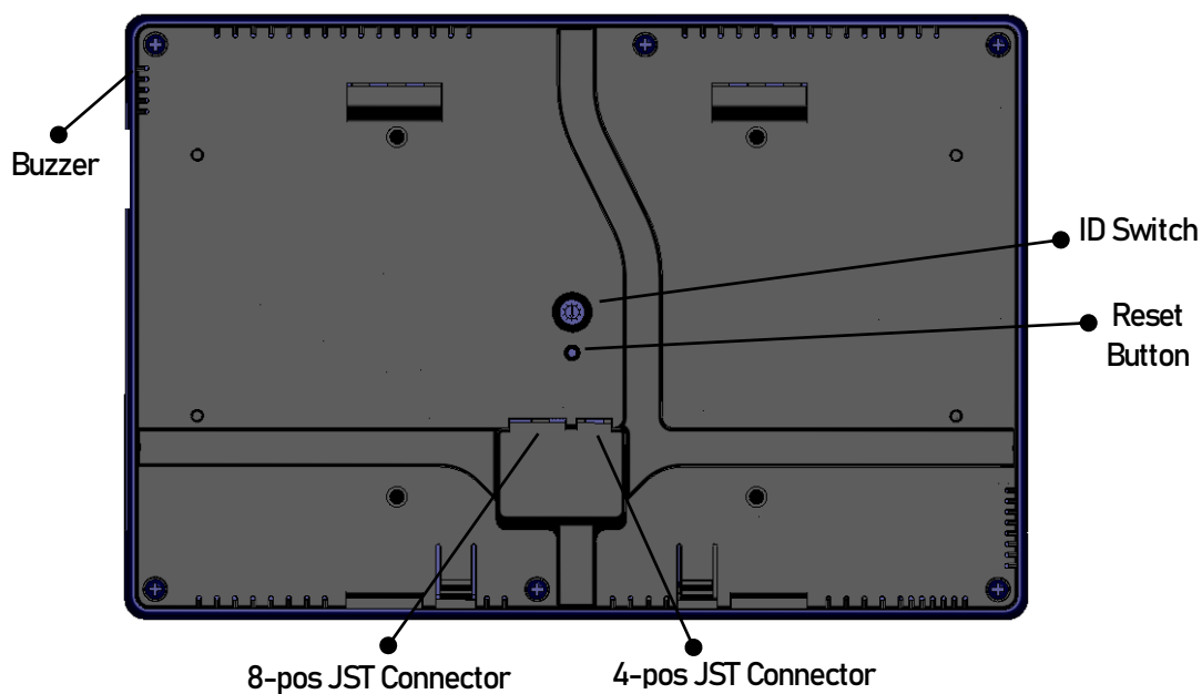
Figure 25 - IDP-1000-04A Display Rear View
