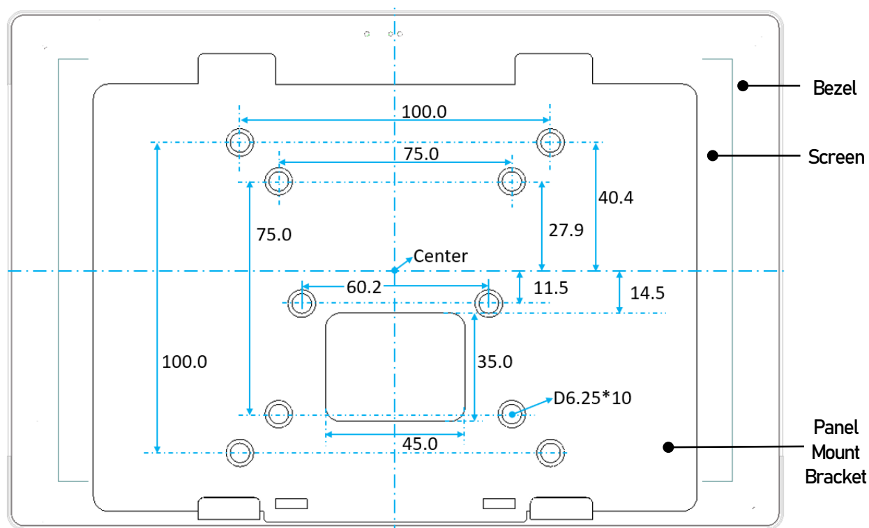
Figure 32 - Panel Mount Bracket Drill Holes Drawings (Front View)
