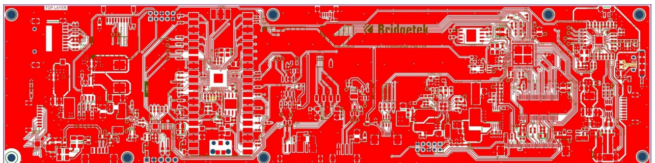
Figure 11 - Main PCB Top Layer
