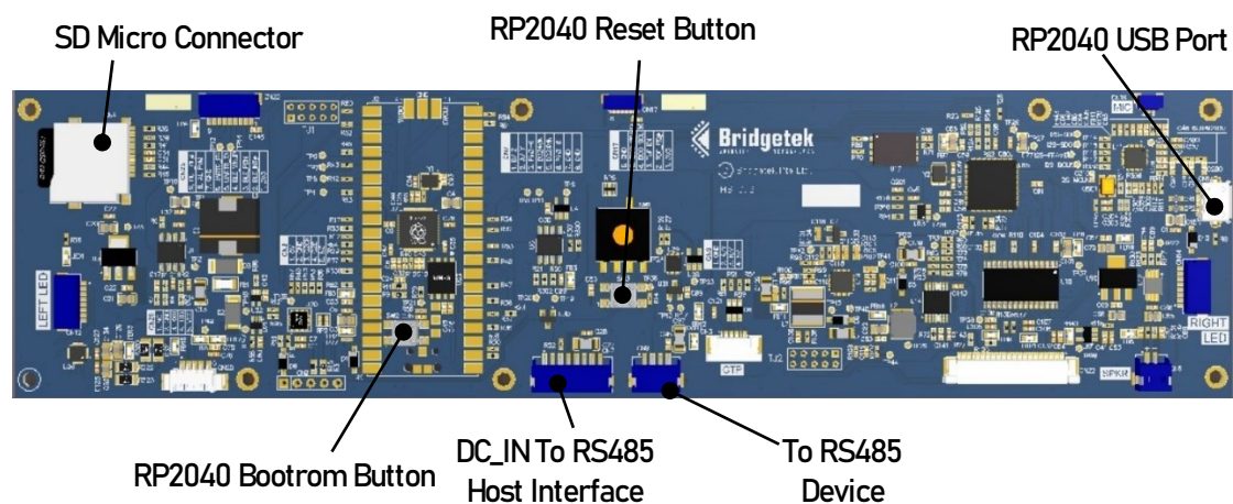
Figure 40 - Debugging and Commonly Use Connectors
