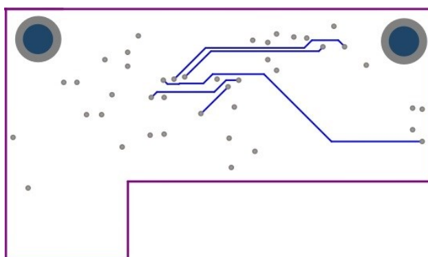
Figure 16 - Sound PCB Bottom Layer
