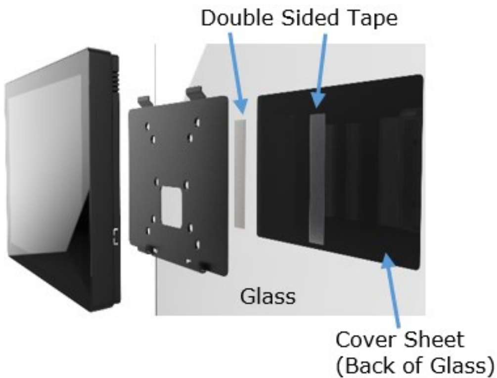
Figure 35 - Glass Mount
