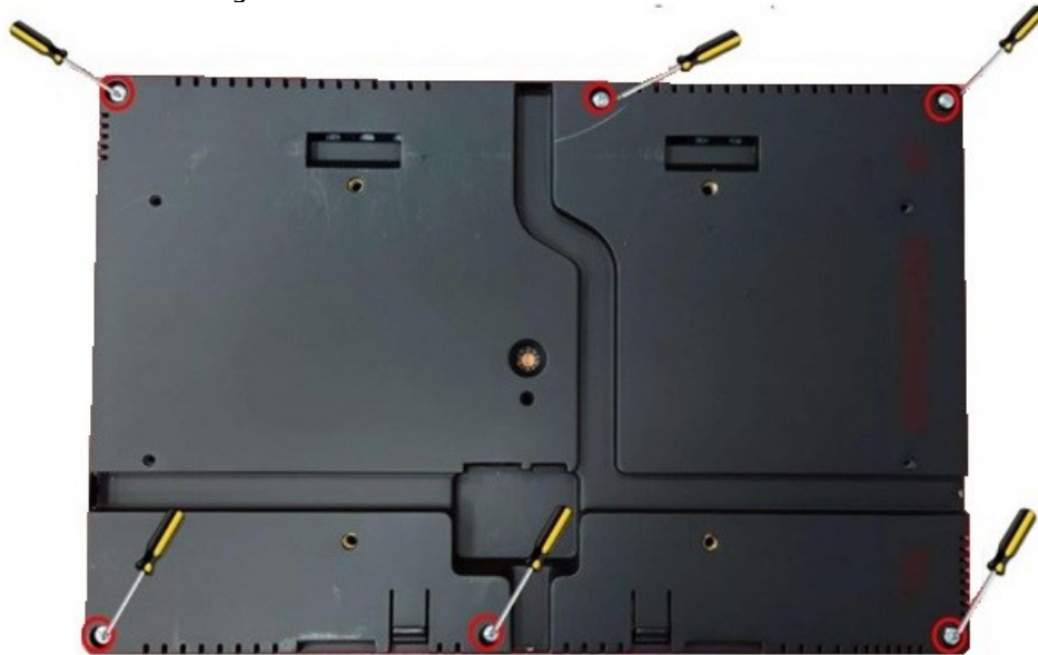
Figure 38 - Remove screws to detach back cover
