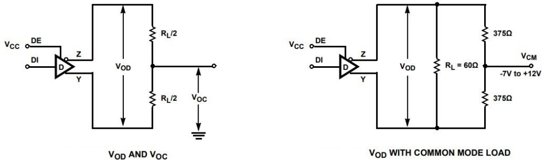
Figure 30 - DC Driver Test Circuits
