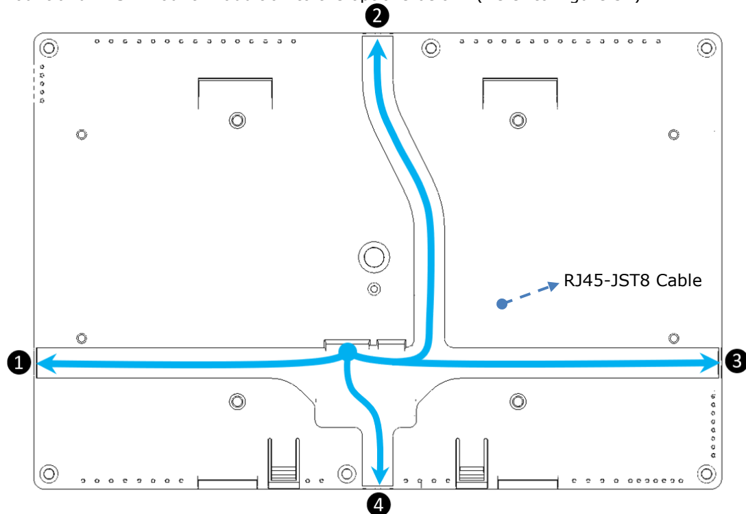
Figure 37 - RJ45-JST8 Cable Wiring Direction Options
