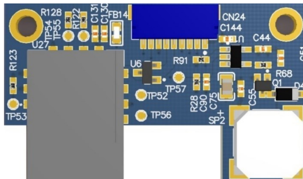
Figure 7 - Sound Board PCBA Front View
