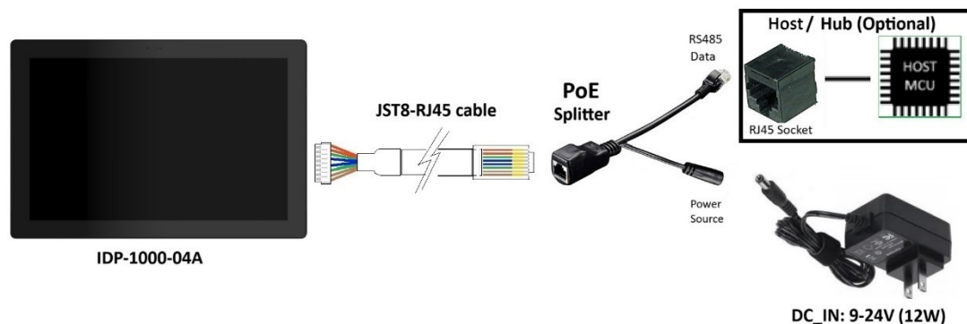
Figure 29 - IDP-1000-04A Connection to Host with Use of PoE Splitter
