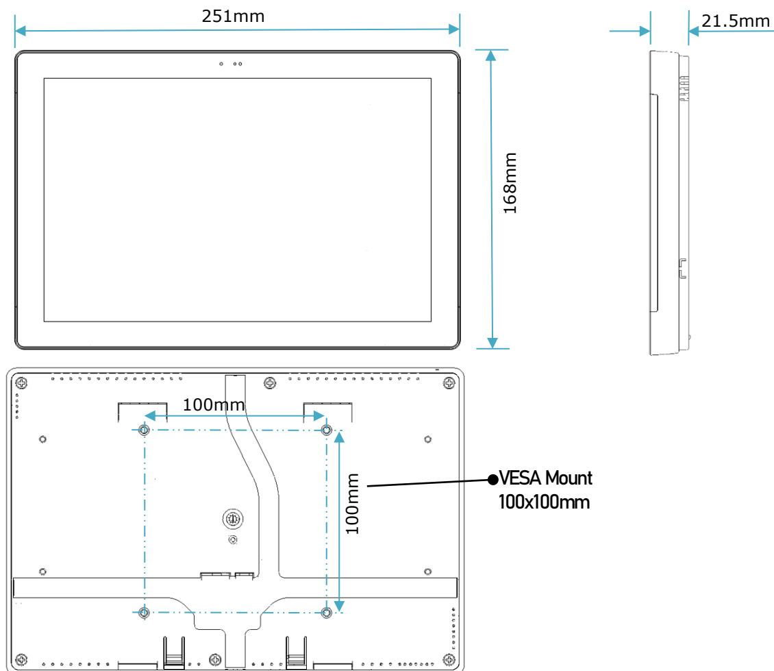
Figure 31 - IDP-1000-04A Display Dimensions
