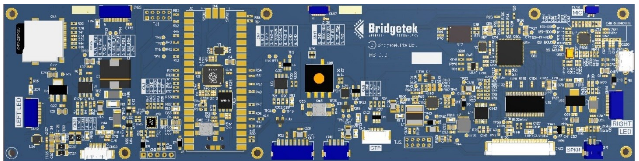
Figure 3 - Mainboard PCBA Front View
