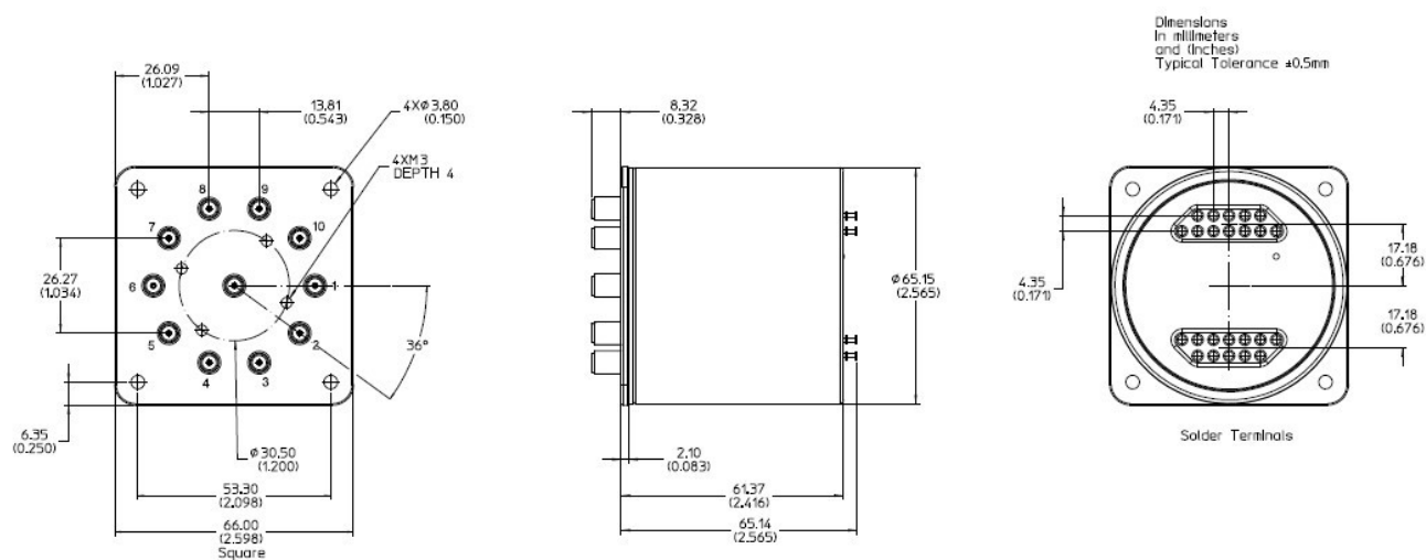
Figure 10. U7110A/B/C mechanical dimension (options 400 and 500) – solder terminal
