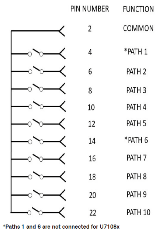
Figure 2. Pin configuration for indicator function
