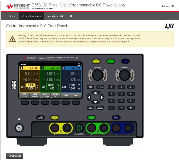
Figure 6 Control the power supply from anywhere with the web graphical user interface which is identical to operating the instrument front panel.
