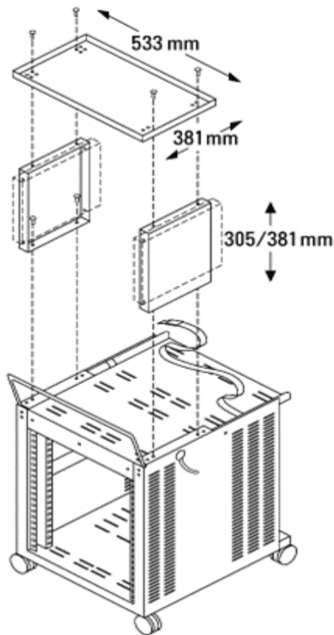
Figure 51. Printer/plotter stand
