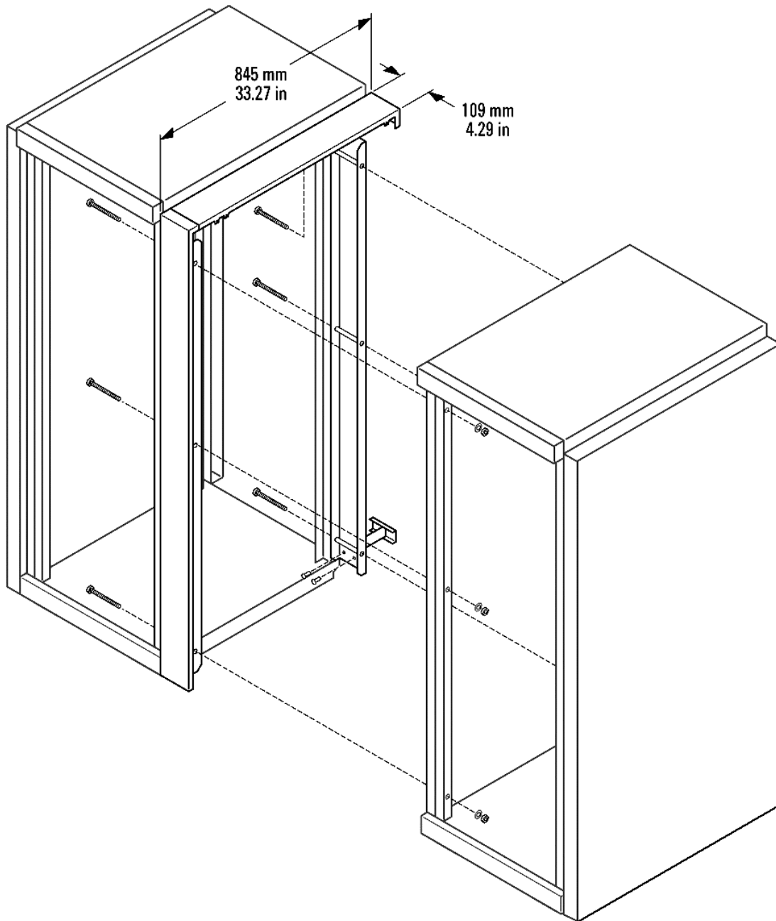
Figure 9. Double-bay configuration
