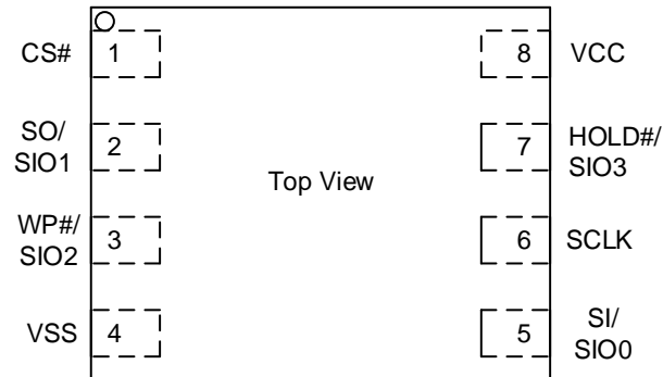
8 - LEAD WSON
