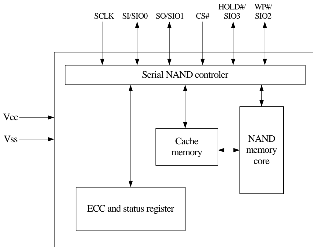
Figure 2-2 Block Diagram
