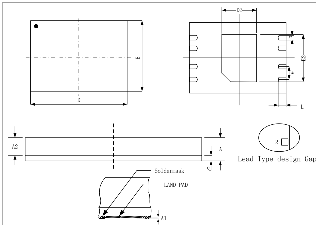
Figure21-4. LGA8 GD Type1 (6*8 mm)
