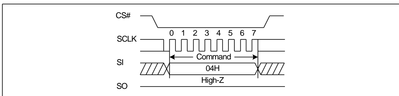
Figure6-2. Write Disable Sequence Diagram
