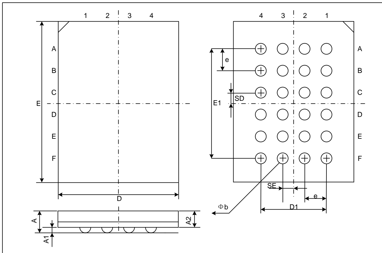
Figure21-3. TFBGA-24BALL (6*4 ball array)
