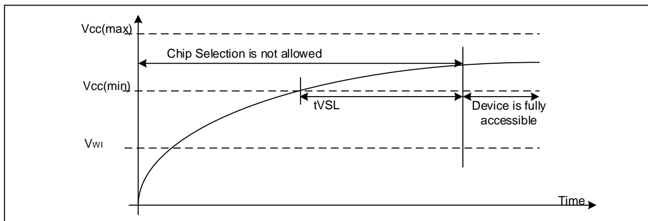
Figure14-1. Power on Timing Sequence
