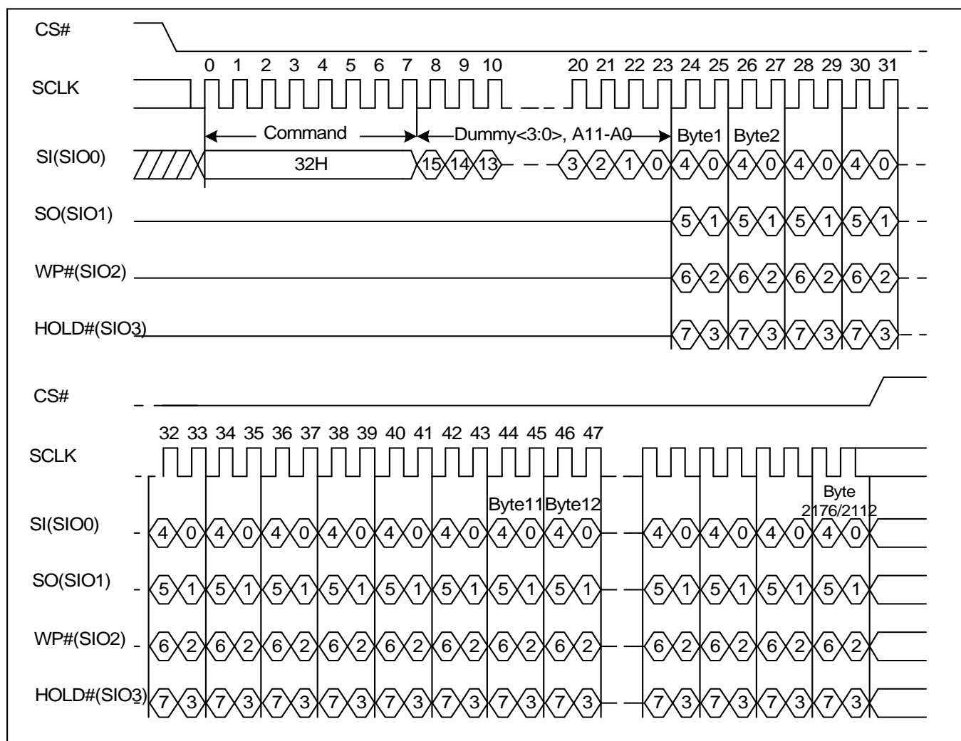
Figure10-2. Program Load x4 Sequence Diagram
