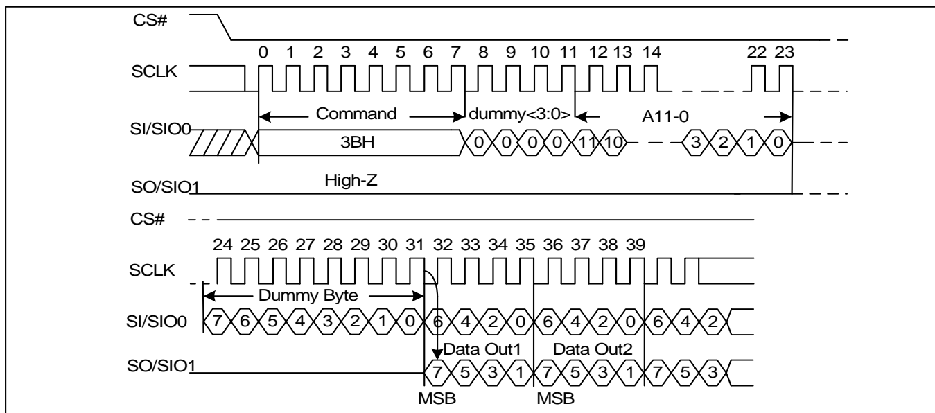
Figure8-3. Read From Cache x2 Sequence Diagram
