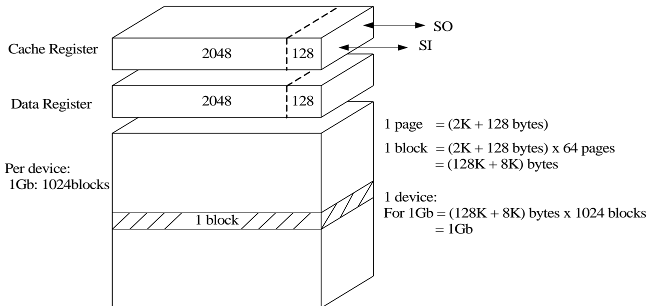
Figure3-1. Array Organization
