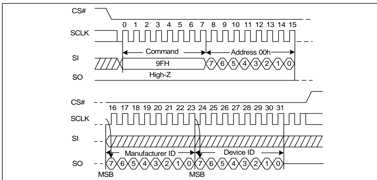
Figure9-1_1. Read ID Sequence Diagram(Address 00h)
