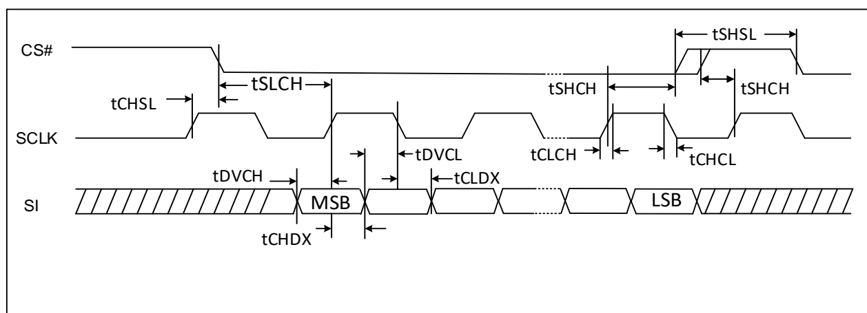
Figure 18-4. Serial Input Timing (DTR)
