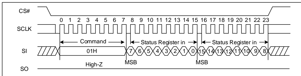
Figure 6. Write Status Register-1&2 Sequence Diagram
