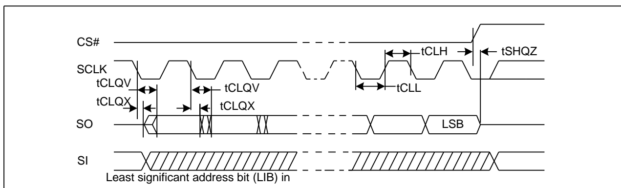
Figure 42. Output Timing
