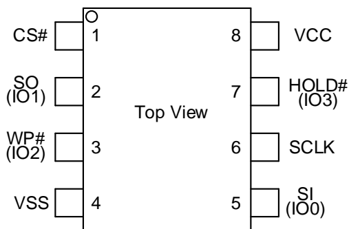
8 - LEAD SOP
