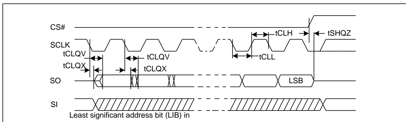
Figure42. Output Timing
