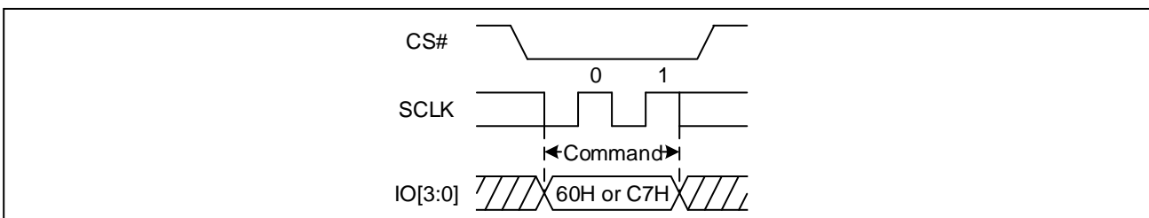
Figure 33. Chip Erase Sequence Diagram (QPI)
