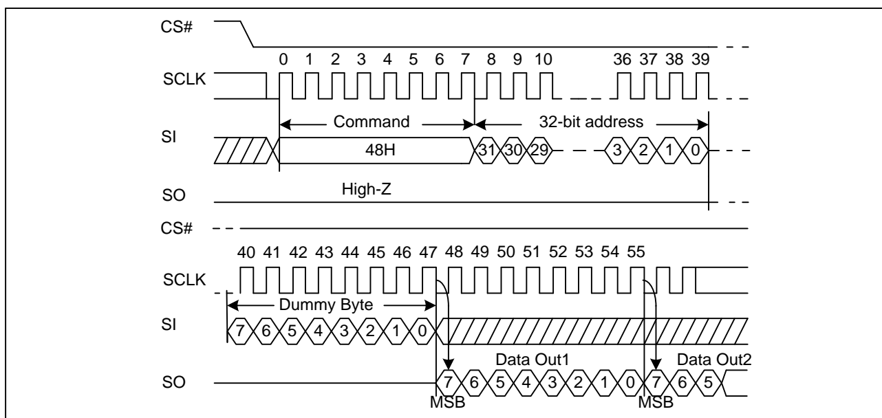
Figure 70 Read Security Registers command Sequence Diagram (ADS=1)
