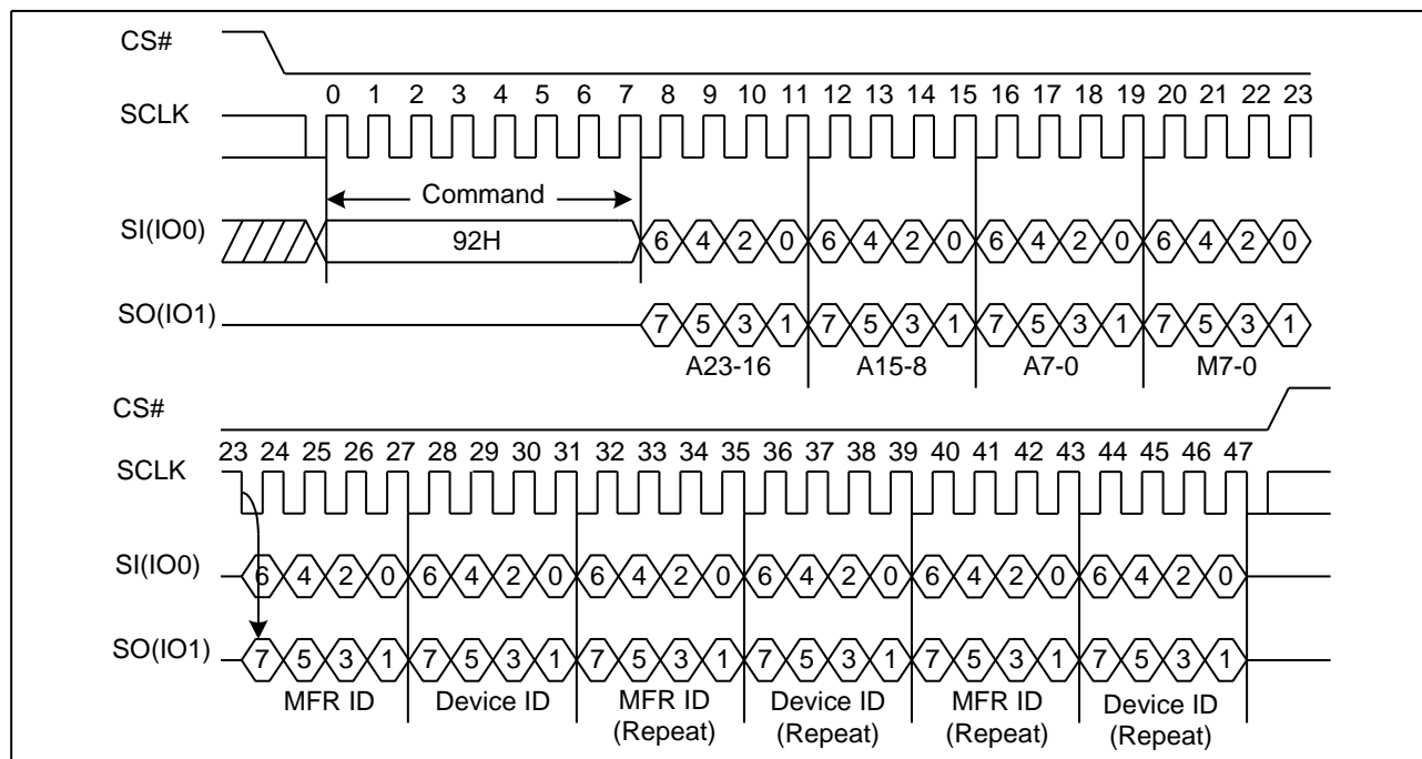
Figure 60. Read ID/ Device ID Dual I/O Sequence Diagram
