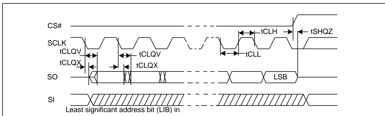
Figure 77 Output Timing
