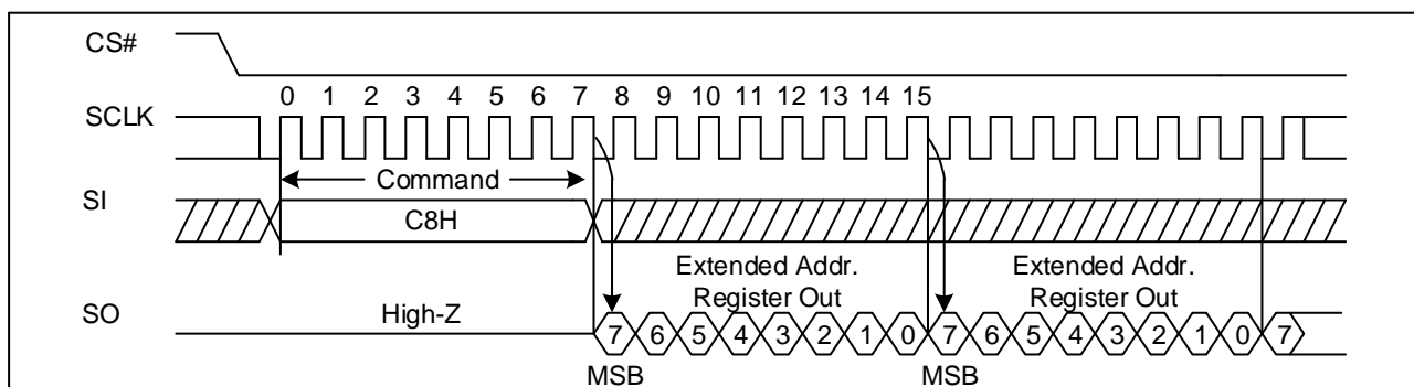
Figure 8 Read Extended Register Sequence Diagram
