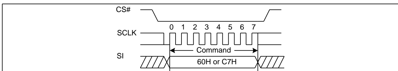
Figure 50 Chip Erase Sequence Diagram
