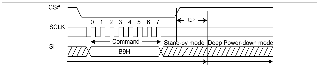
Figure 51 Deep Power-Down Sequence Diagram
