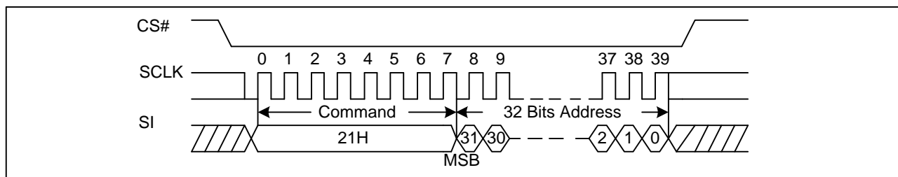
Figure 43 Sector Erase with 4-Byte Address Sequence Diagram (ADS=0 or ADS=1)
