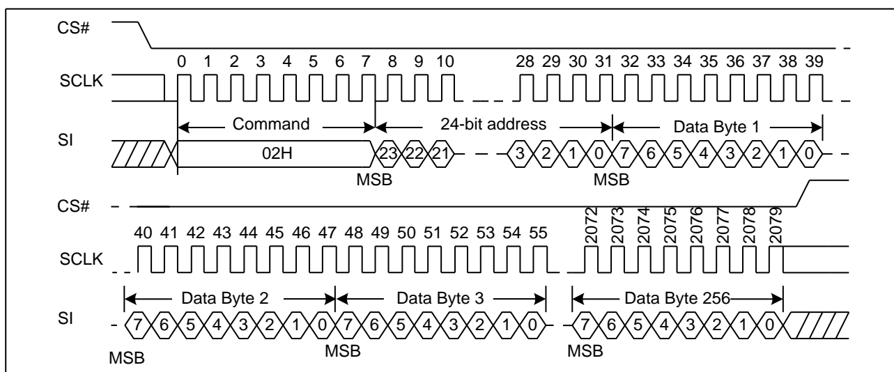
Figure 35 Page Program Sequence Diagram (ADS=0)
