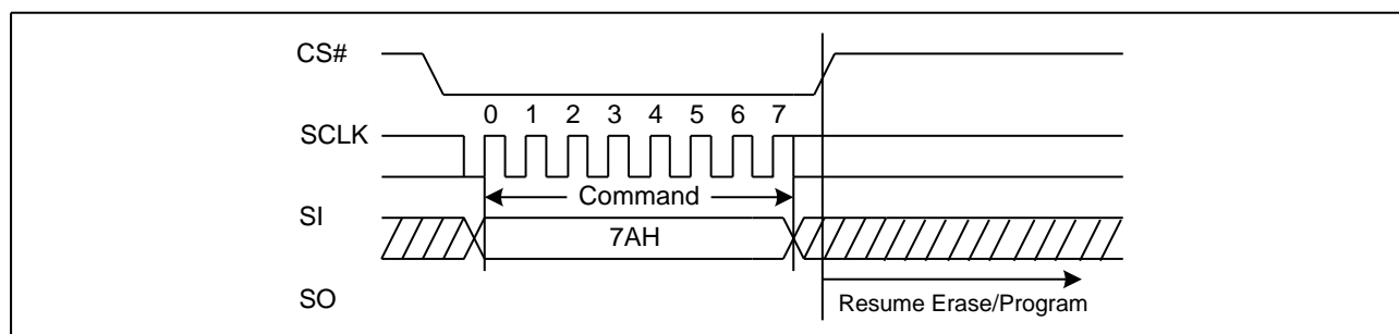
Figure 64 Program/Erase Resume Sequence Diagram
