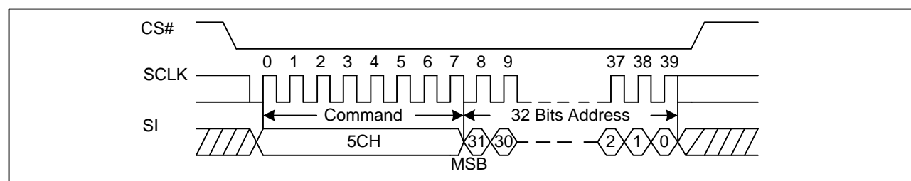
Figure 46 32KB Block Erase with 4-Byte Address Sequence Diagram (ADS=0 or ADS=1)
