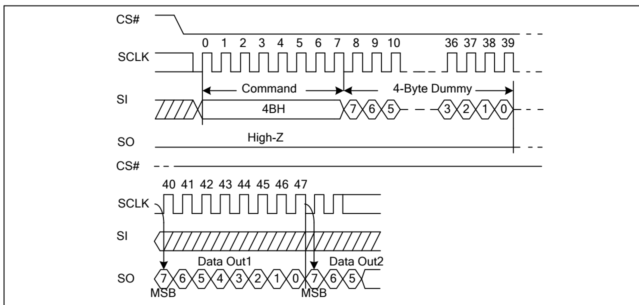
Figure 53 Read Unique ID Sequence Diagram (ADS=1)
