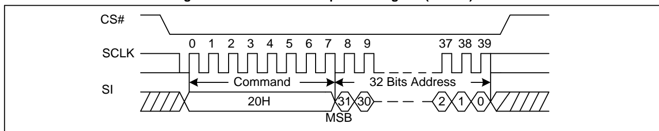
Figure 42 Sector Erase Sequence Diagram (ADS=1)
