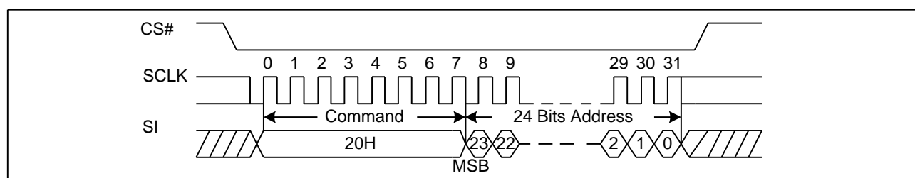
Figure 41 Sector Erase Sequence Diagram (ADS=0)
