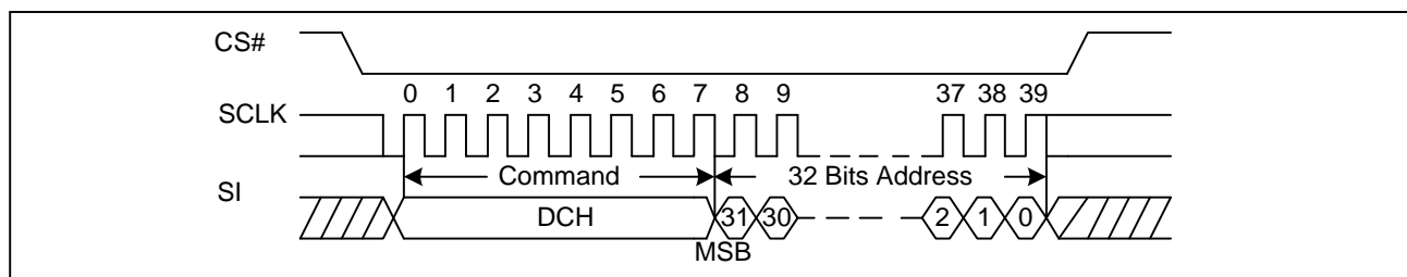
Figure 49 64KB Block Erase with 4-Byte Address Sequence Diagram (ADS=0 or ADS=1)
