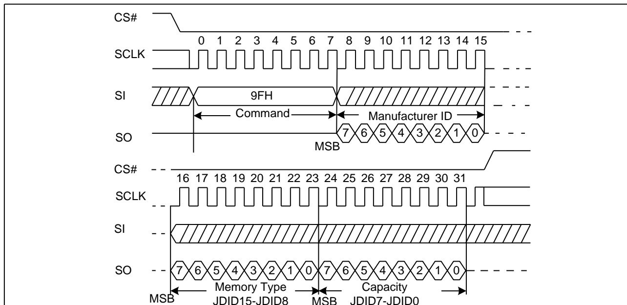
Figure 62 Read Identification ID Sequence Diagram
