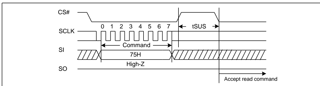
Figure 63 Program/Erase Suspend Sequence Diagram
