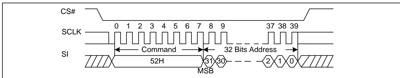
Figure 45 32KB Block Erase Sequence Diagram (ADS=1)
