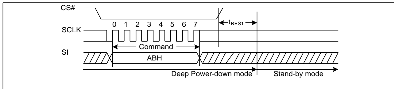
Figure 57 Release Power-Down Sequence Diagram
