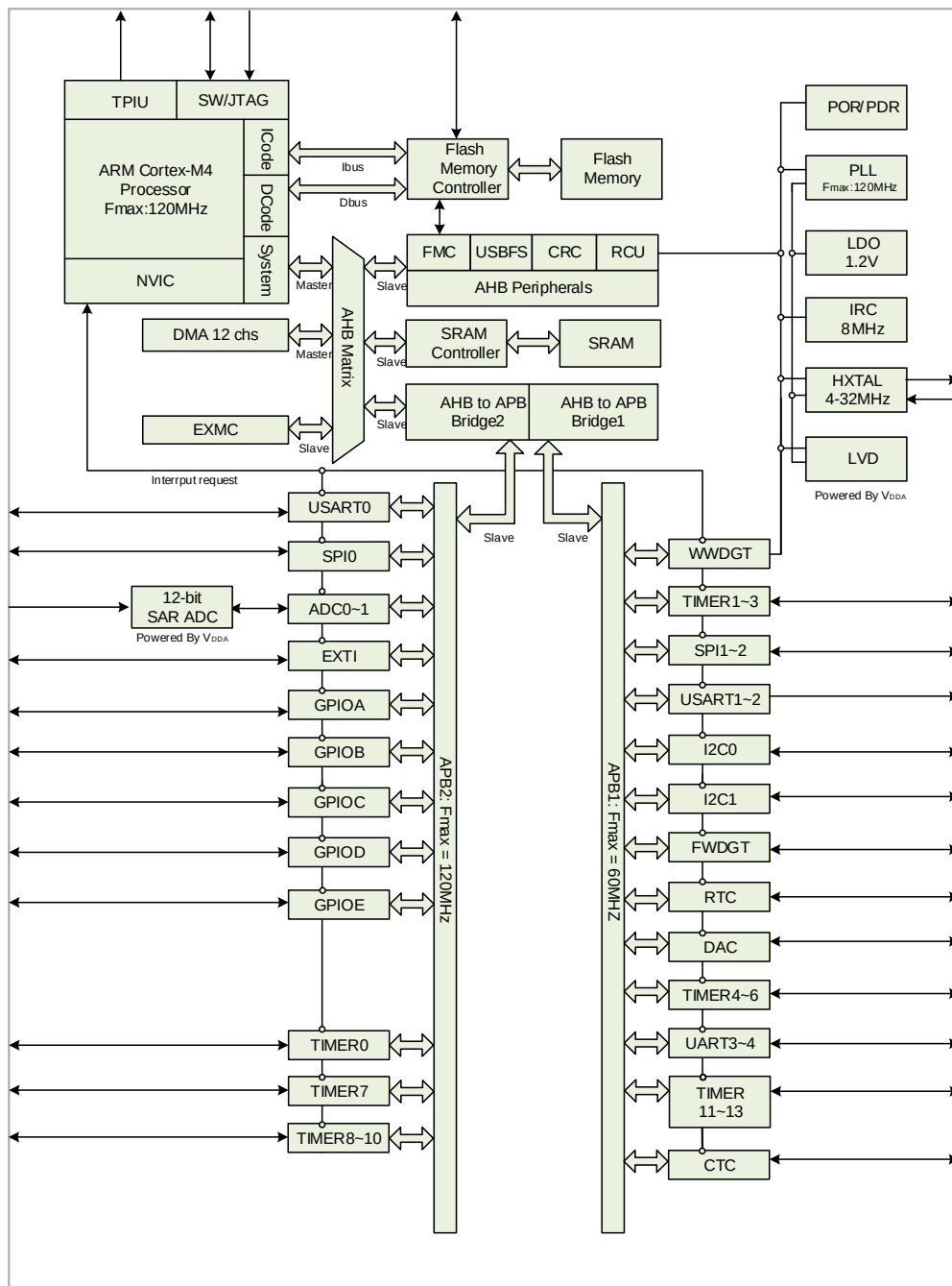
Figure 2-1.GD32E103xx block diagram
