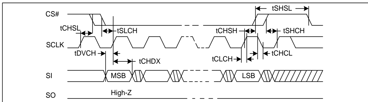
Figure 25. Input Timing
