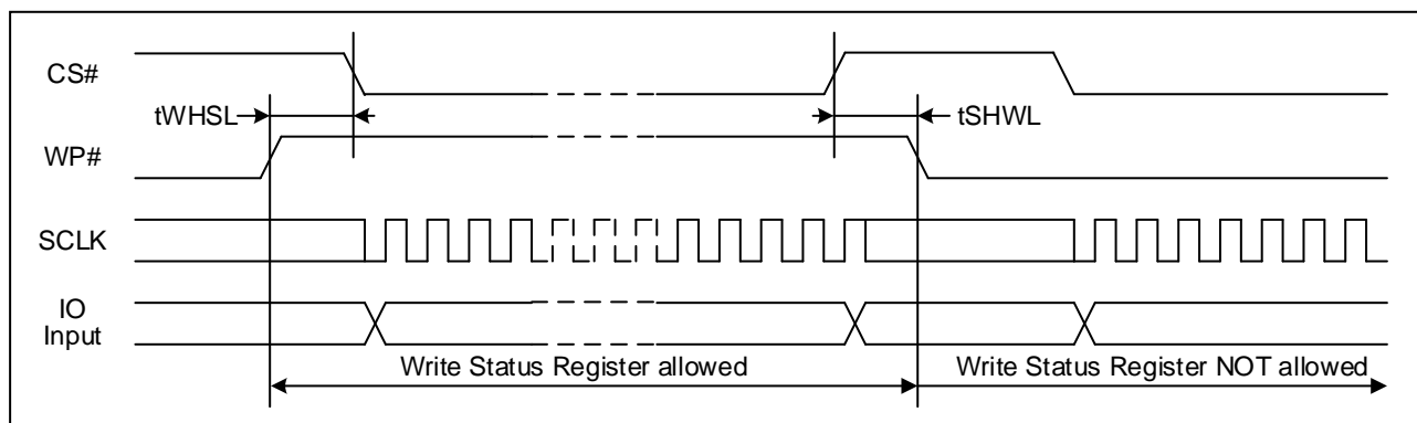
Figure 44. WP# Timing
