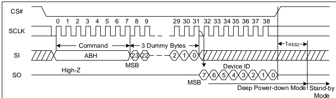
Figure 35. Release Power-Down/Read Device ID Sequence Diagram
