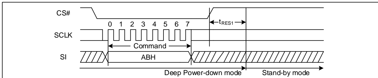
Figure 34. Release Power-Down Sequence Diagram
