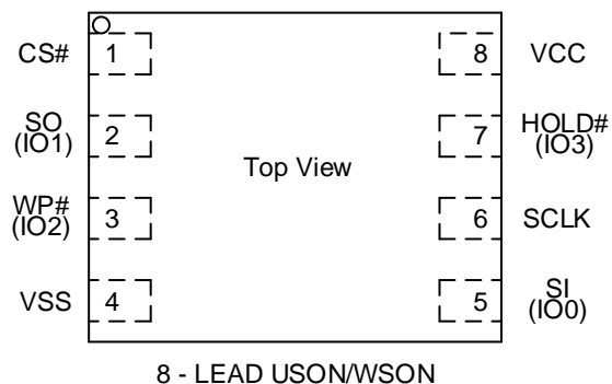
Figure 2 Connection Diagram for USON8/WSN8 Package
