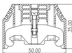
Dimensions — mm
