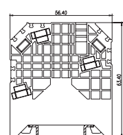
Dimensions — mm
