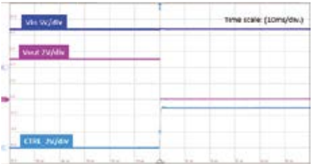
Figure 9: CNTRL high level, DC-DC off
