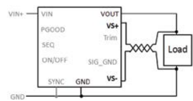
Figure 5: Voltage sense configuration
