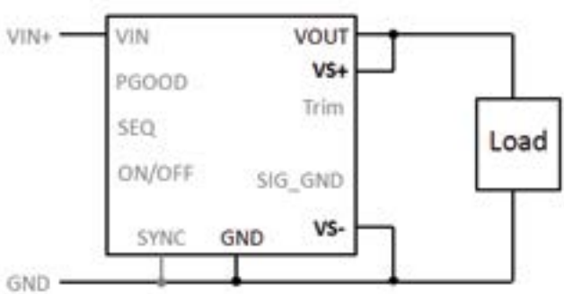
Figure 6: No voltage sense configuration
