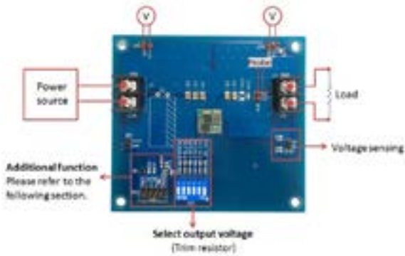
Figure 2: Test set-up example
