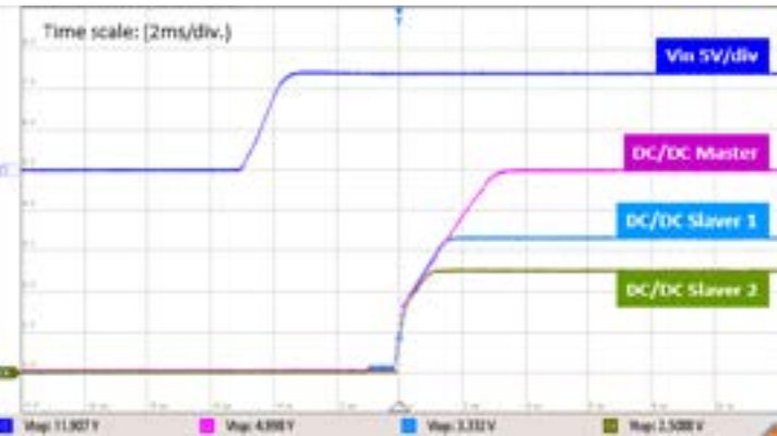
Figure 18: Sequencing curve
