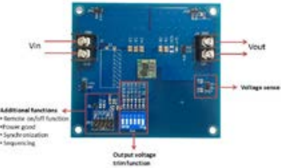
Figure 1. EPM12V2 EVK
