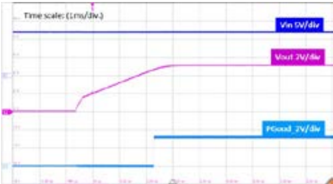
Figure 16: PG000 curve
