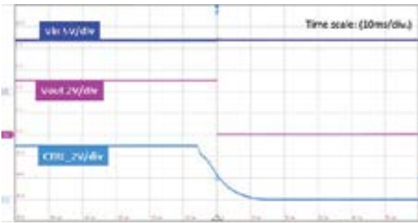
Figure 11: CNTRL low level, DC-DC off
