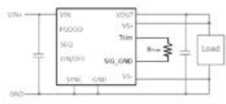
Figure 3: Voltage trim resistor diagram
