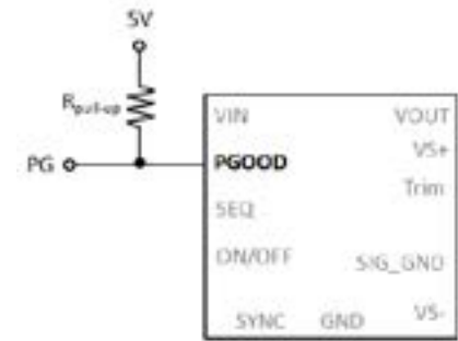
Figure 15: PG000 circuit diagram
