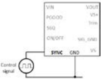
Figure 12: External signal to SYNC circuit diagram
