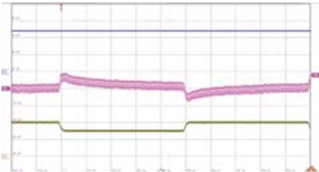
Ch1: Input voltage (5 V/div.) Ch4: Output current (0.5 A/div) Ch2: Output voltage (20 mV/div.) Time scale: (100 us/div.)
