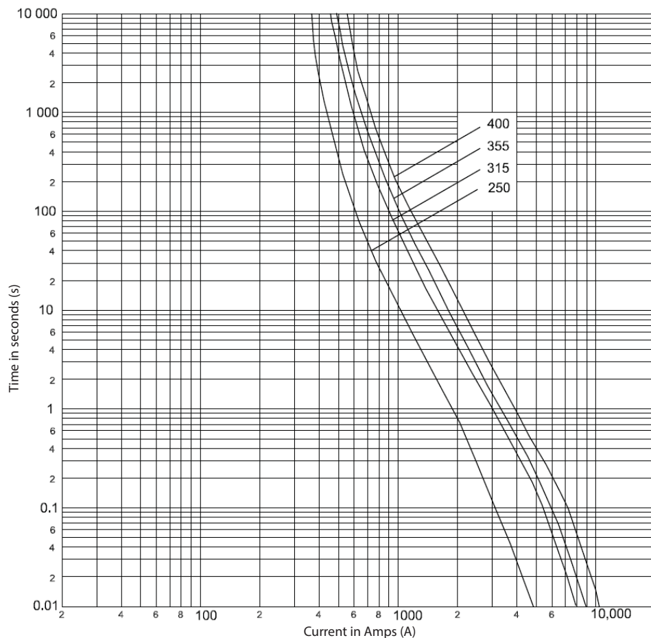
Time-current curves - NH Size 03
