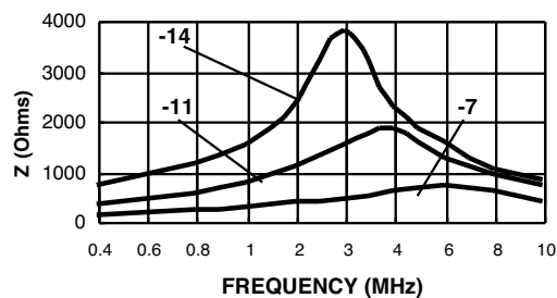
Impedance CMS1 - 7,11, & 14
