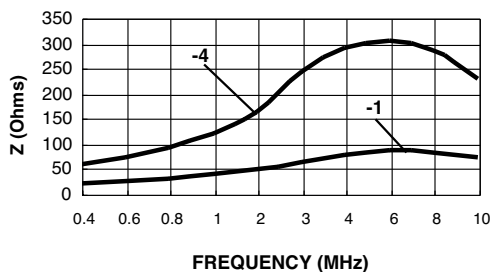
Impedance CMS1-1 & 4
