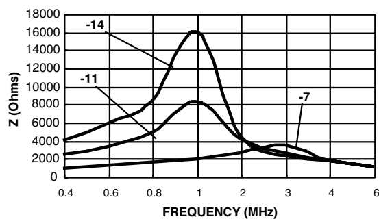
Impedance CMS3 - 7,11, & 14
