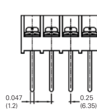
04 Wire Wrap Tail
