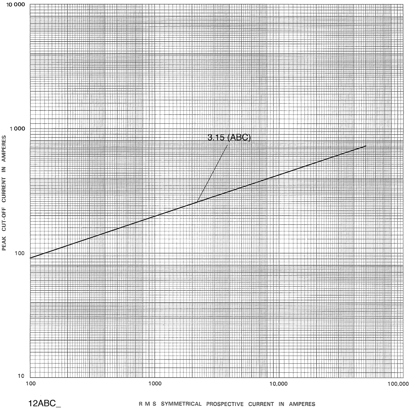
12 kV peak let-through curves for 12ABC_
