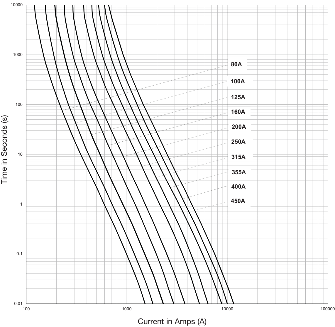
Time-Current Characteristics - TCP80 to TCP100 and TFP125 to TFP200
