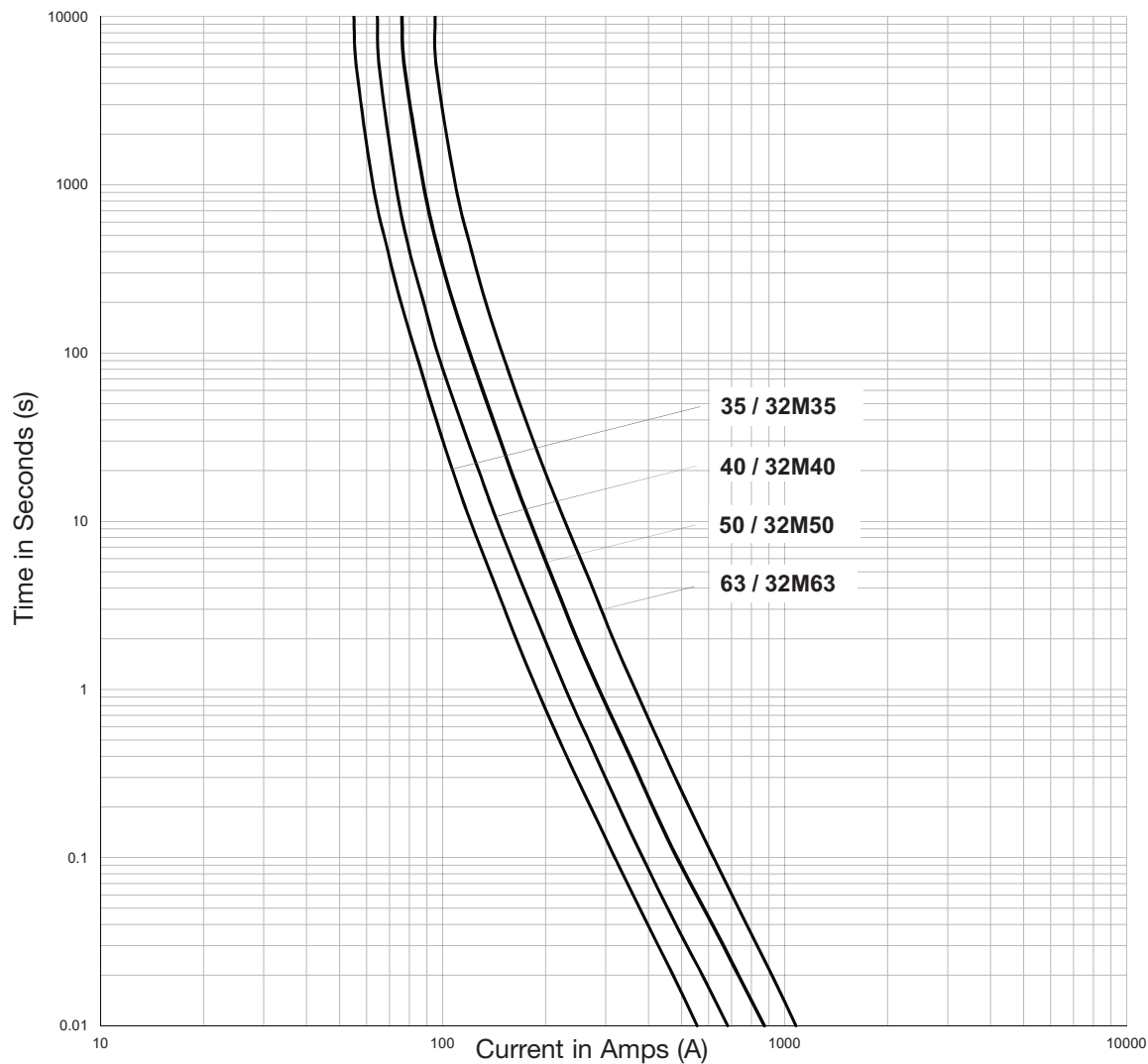
Time-Current Characteristics - TIA32M, TIS35 to TIS63 and TCP40 to TCP63
