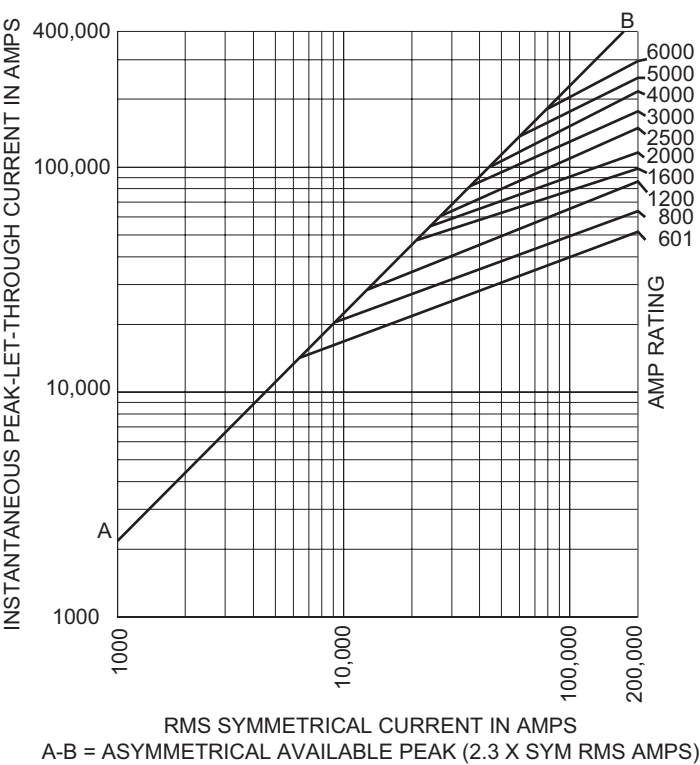
Current-limitation curves
