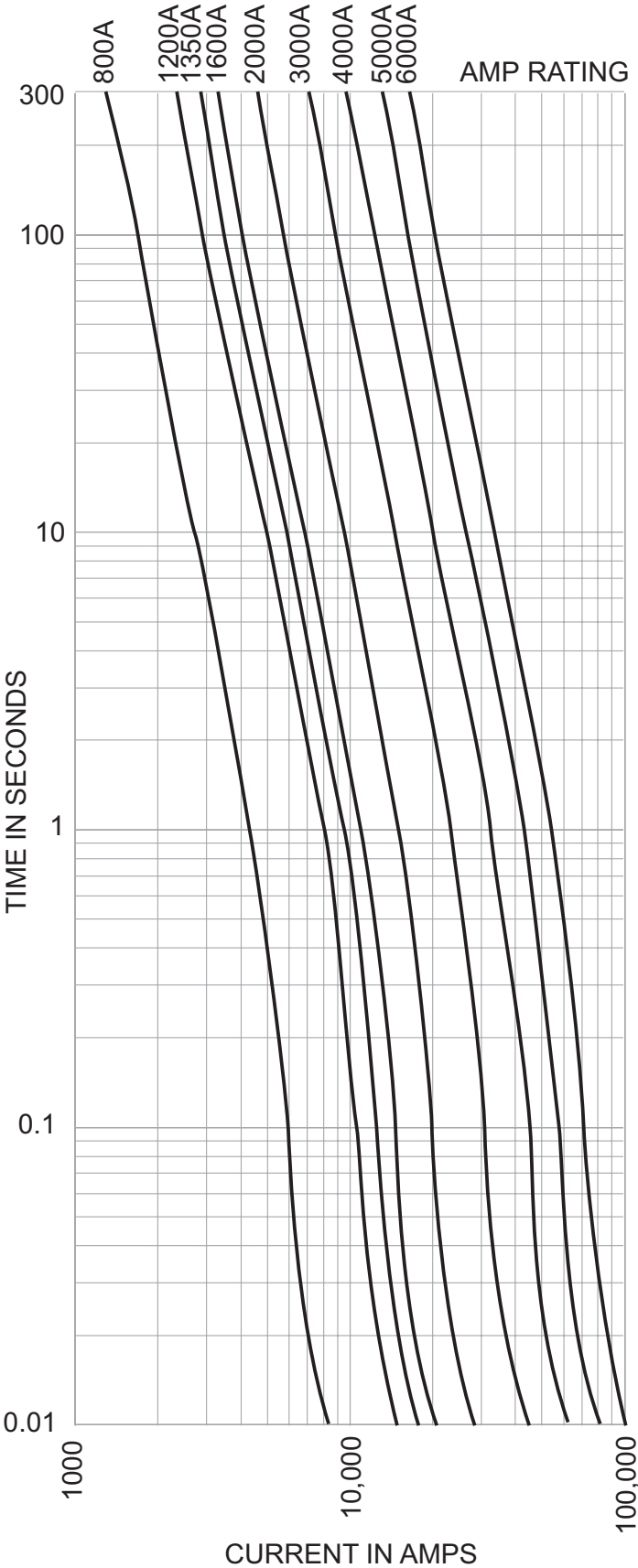
Time-current curves - average melt
